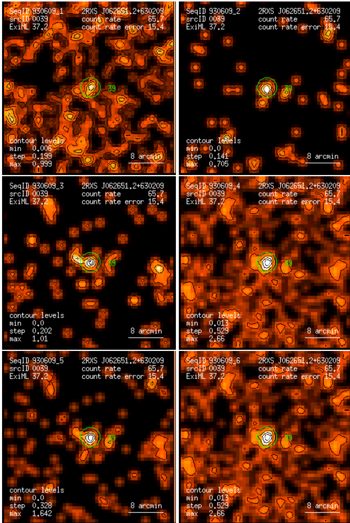
Figure 39: RASS 930609: detection 0039: band rate images, Gaussian filter: (1) PSPC channels 11 – 41, (2) 52 – 90, (3) 91 – 201, (4) 11 – 235, (5) 52 – 201, (6) 11 – 201. Broad band rates in counts/ks. Band rate contour levels in counts/ks/arcmin 2 .
