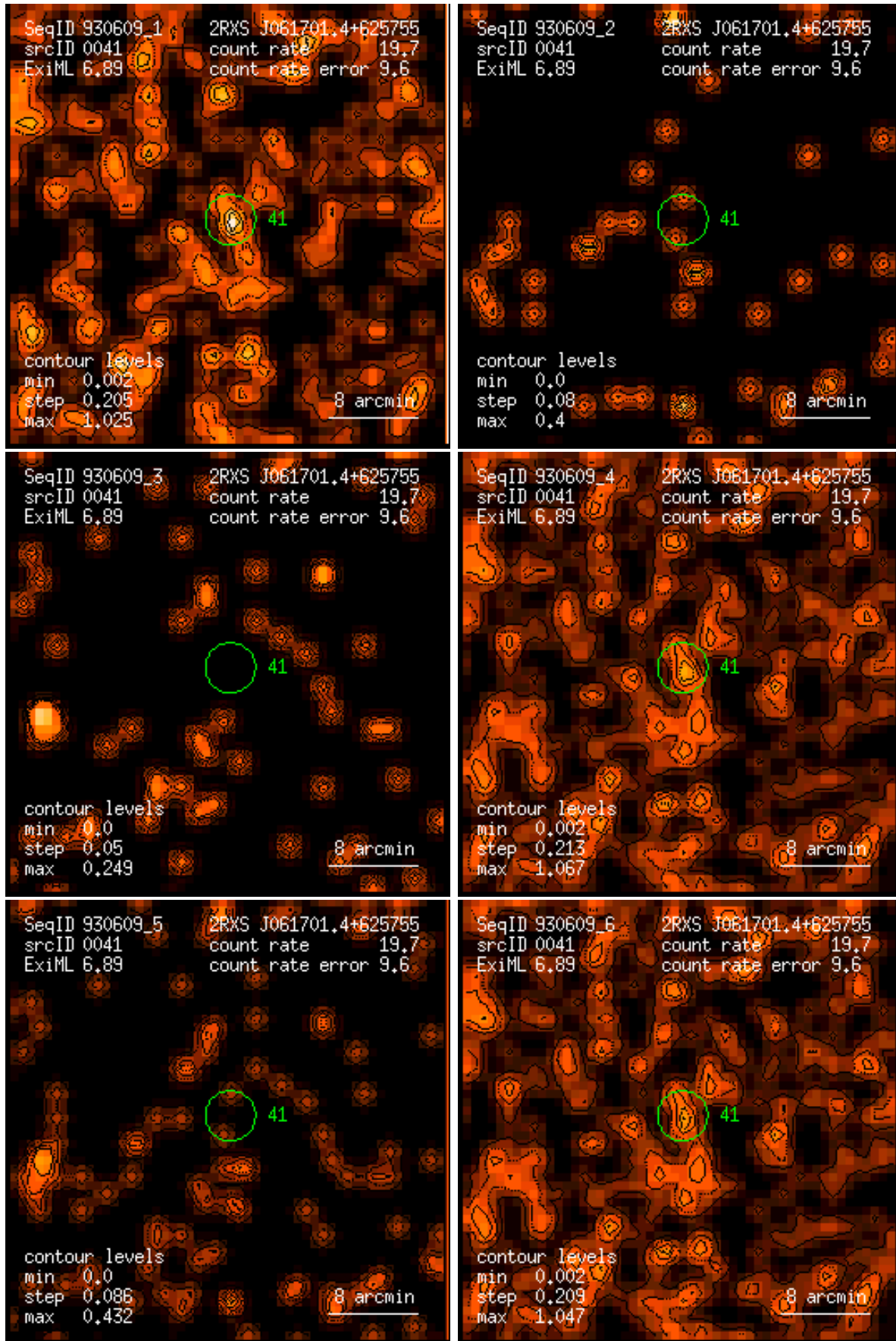
Figure 41: RASS 930609: detection 0041: band rate images, Gaussian filter: (1) PSPC channels 11 – 41, (2) 52 – 90, (3) 91 – 201, (4) 11 – 235, (5) 52 – 201, (6) 11 – 201. Broad band rates in counts/ks. Band rate contour levels in counts/ks/arcmin 2 .
