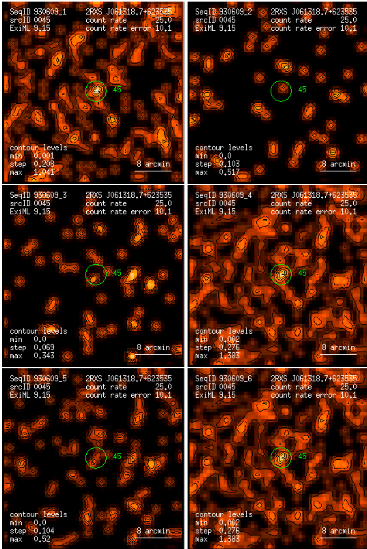
Figure 45: RASS 930609: detection 0045: band rate images, Gaussian filter: (1) PSPC channels 11 – 41, (2) 52 – 90, (3) 91 – 201, (4) 11 – 235, (5) 52 – 201, (6) 11 – 201. Broad band rates in counts/ks. Band rate contour levels in counts/ks/arcmin 2 .
