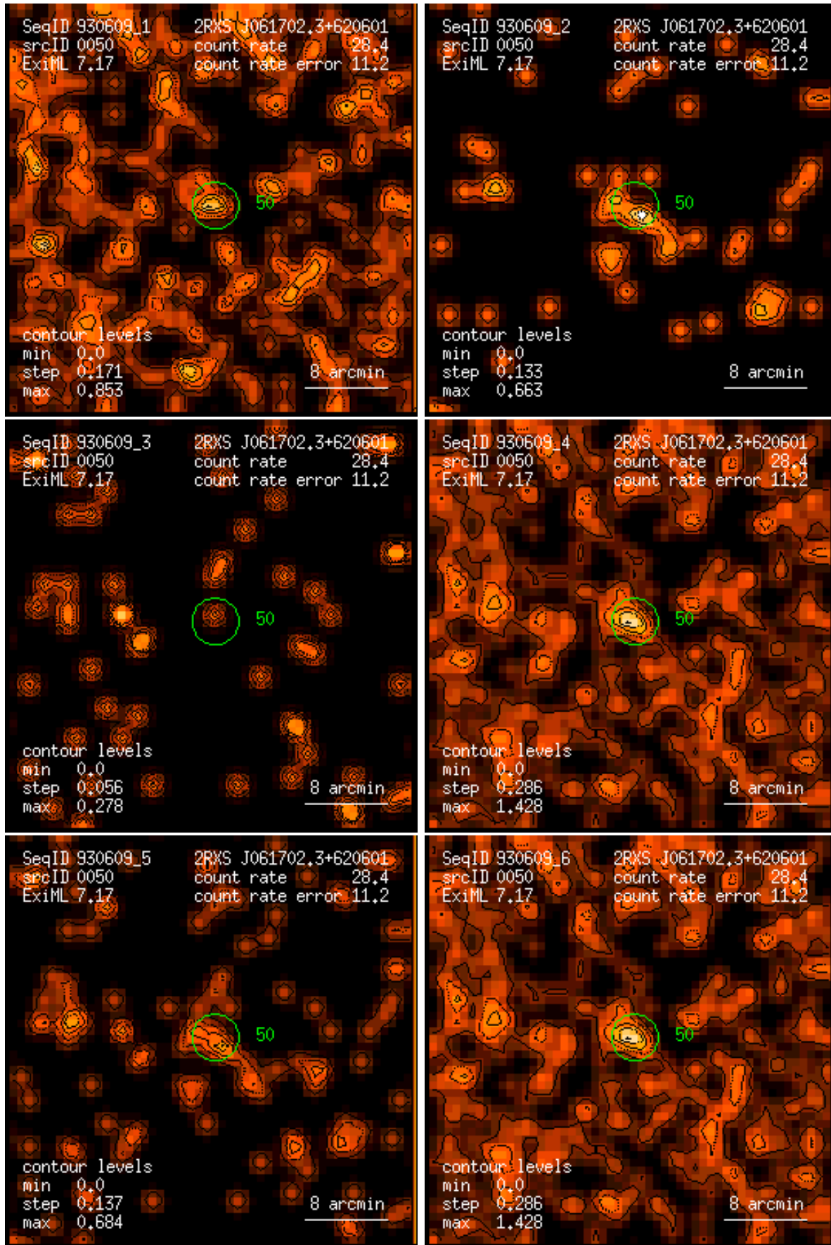
Figure 50: RASS 930609: detection 0050: band rate images, Gaussian filter: (1) PSPC channels 11 – 41, (2) 52 – 90, (3) 91 – 201, (4) 11 – 235, (5) 52 – 201, (6) 11 – 201. Broad band rates in counts/ks. Band rate contour levels in counts/ks/arcmin 2 .
