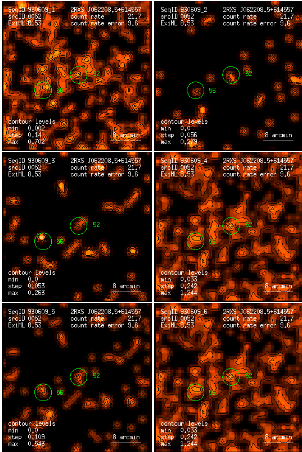
Figure 52: RASS 930609: detection 0052: band rate images, Gaussian filter: (1) PSPC channels 11 – 41, (2) 52 – 90, (3) 91 – 201, (4) 11 – 235, (5) 52 – 201, (6) 11 – 201. Broad band rates in counts/ks. Band rate contour levels in counts/ks/arcmin 2 .
