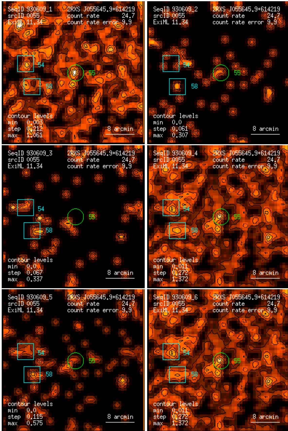
Figure 55: RASS 930609: detection 0055: band rate images, Gaussian filter: (1) PSPC channels 11 – 41, (2) 52 – 90, (3) 91 – 201, (4) 11 – 235, (5) 52 – 201, (6) 11 – 201. Broad band rates in counts/ks. Band rate contour levels in counts/ks/arcmin 2 .
