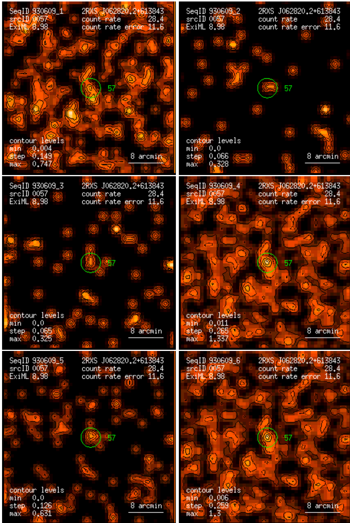
Figure 57: RASS 930609: detection 0057: band rate images, Gaussian filter: (1) PSPC channels 11 – 41, (2) 52 – 90, (3) 91 – 201, (4) 11 – 235, (5) 52 – 201, (6) 11 – 201. Broad band rates in counts/ks. Band rate contour levels in counts/ks/arcmin 2 .
