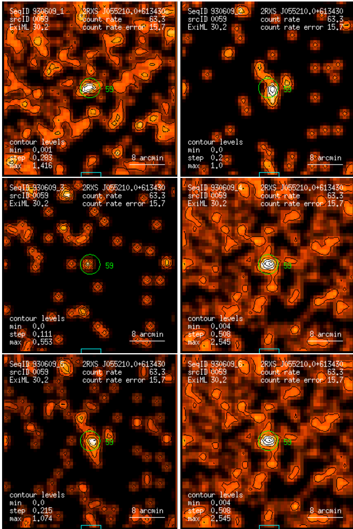
Figure 59: RASS 930609: detection 0059: band rate images, Gaussian filter: (1) PSPC channels 11 – 41, (2) 52 – 90, (3) 91 – 201, (4) 11 – 235, (5) 52 – 201, (6) 11 – 201. Broad band rates in counts/ks. Band rate contour levels in counts/ks/arcmin 2 .
