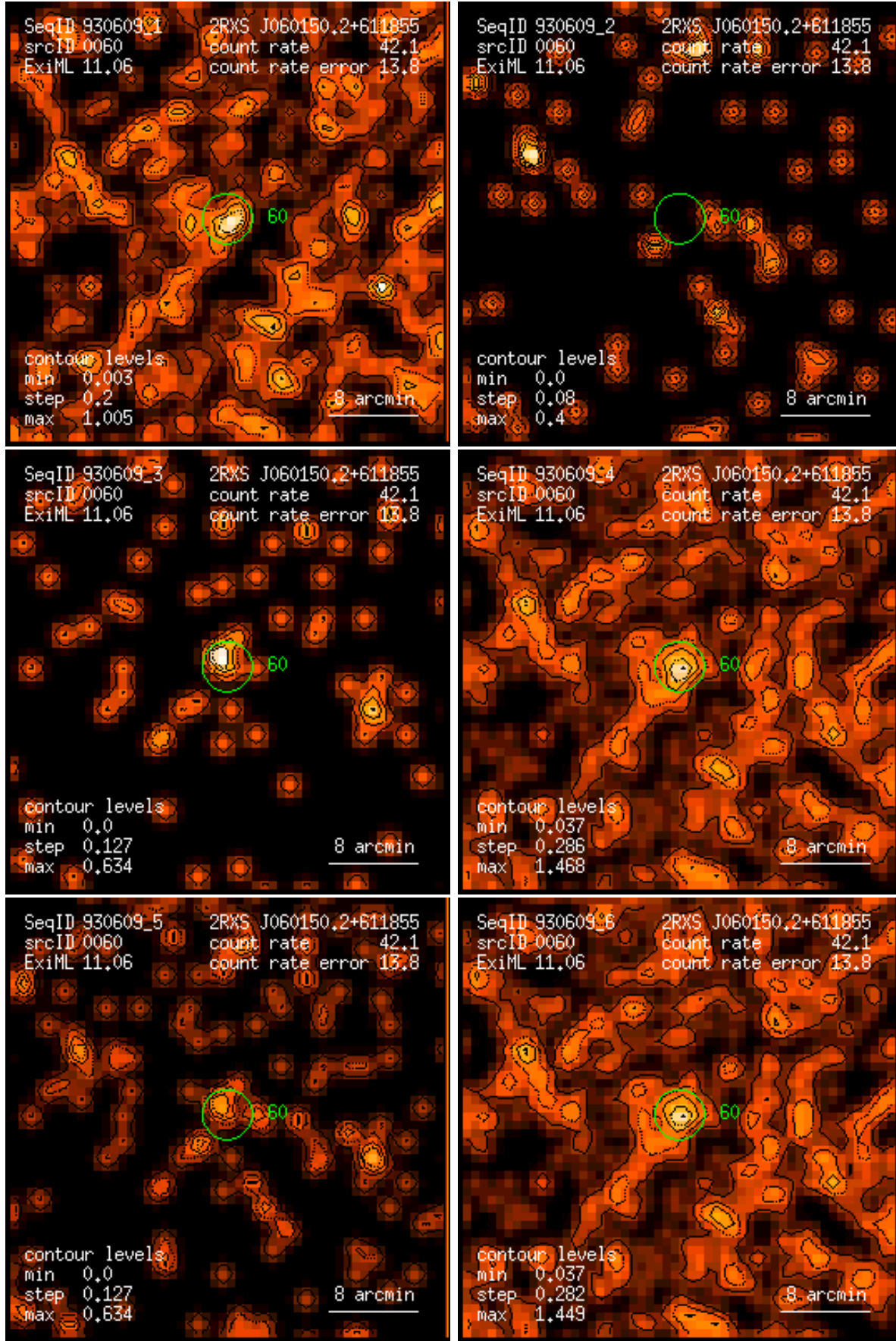
Figure 60: RASS 930609: detection 0060: band rate images, Gaussian filter: (1) PSPC channels 11 – 41, (2) 52 – 90, (3) 91 – 201, (4) 11 – 235, (5) 52 – 201, (6) 11 – 201. Broad band rates in counts/ks. Band rate contour levels in counts/ks/arcmin 2 .
