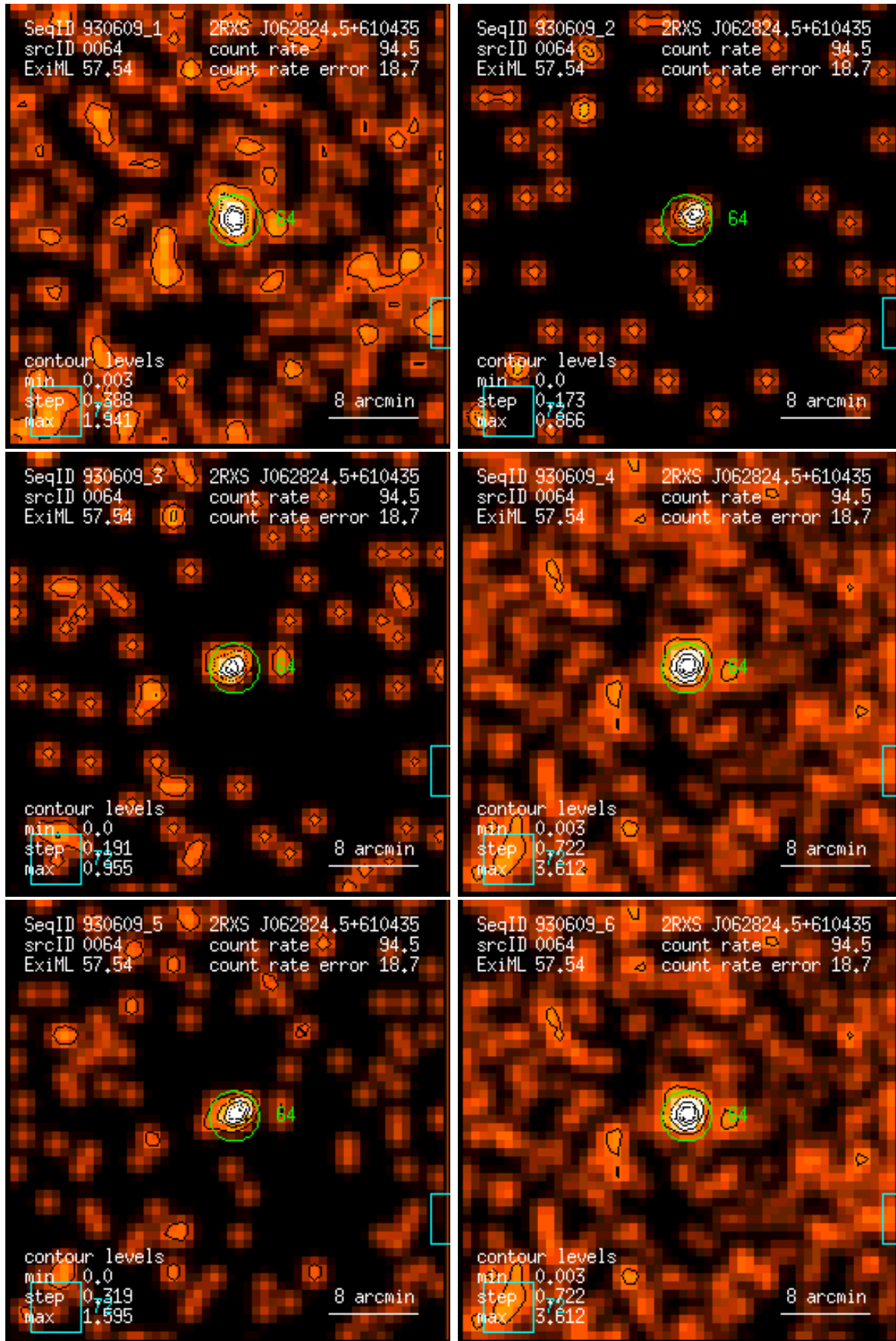
Figure 64: RASS 930609: detection 0064: band rate images, Gaussian filter: (1) PSPC channels 11 – 41, (2) 52 – 90, (3) 91 – 201, (4) 11 – 235, (5) 52 – 201, (6) 11 – 201. Broad band rates in counts/ks. Band rate contour levels in counts/ks/arcmin 2 .
