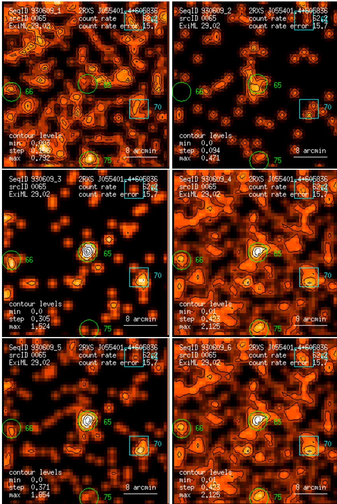
Figure 65: RASS 930609: detection 0065: band rate images, Gaussian filter: (1) PSPC channels 11 – 41, (2) 52 – 90, (3) 91 – 201, (4) 11 – 235, (5) 52 – 201, (6) 11 – 201. Broad band rates in counts/ks. Band rate contour levels in counts/ks/arcmin 2 .
