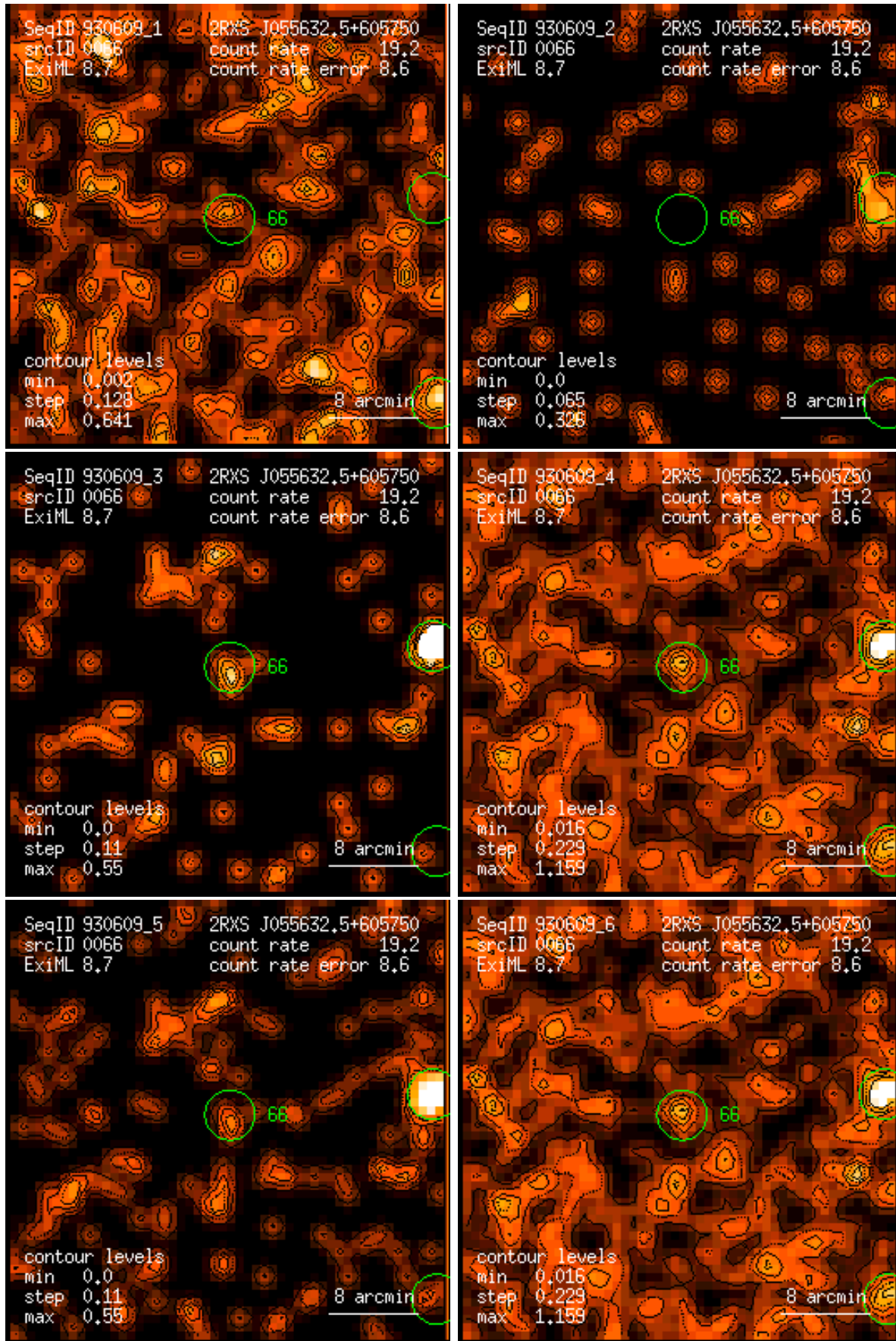
Figure 66: RASS 930609: detection 0066: band rate images, Gaussian filter: (1) PSPC channels 11 – 41, (2) 52 – 90, (3) 91 – 201, (4) 11 – 235, (5) 52 – 201, (6) 11 – 201. Broad band rates in counts/ks. Band rate contour levels in counts/ks/arcmin 2 .
