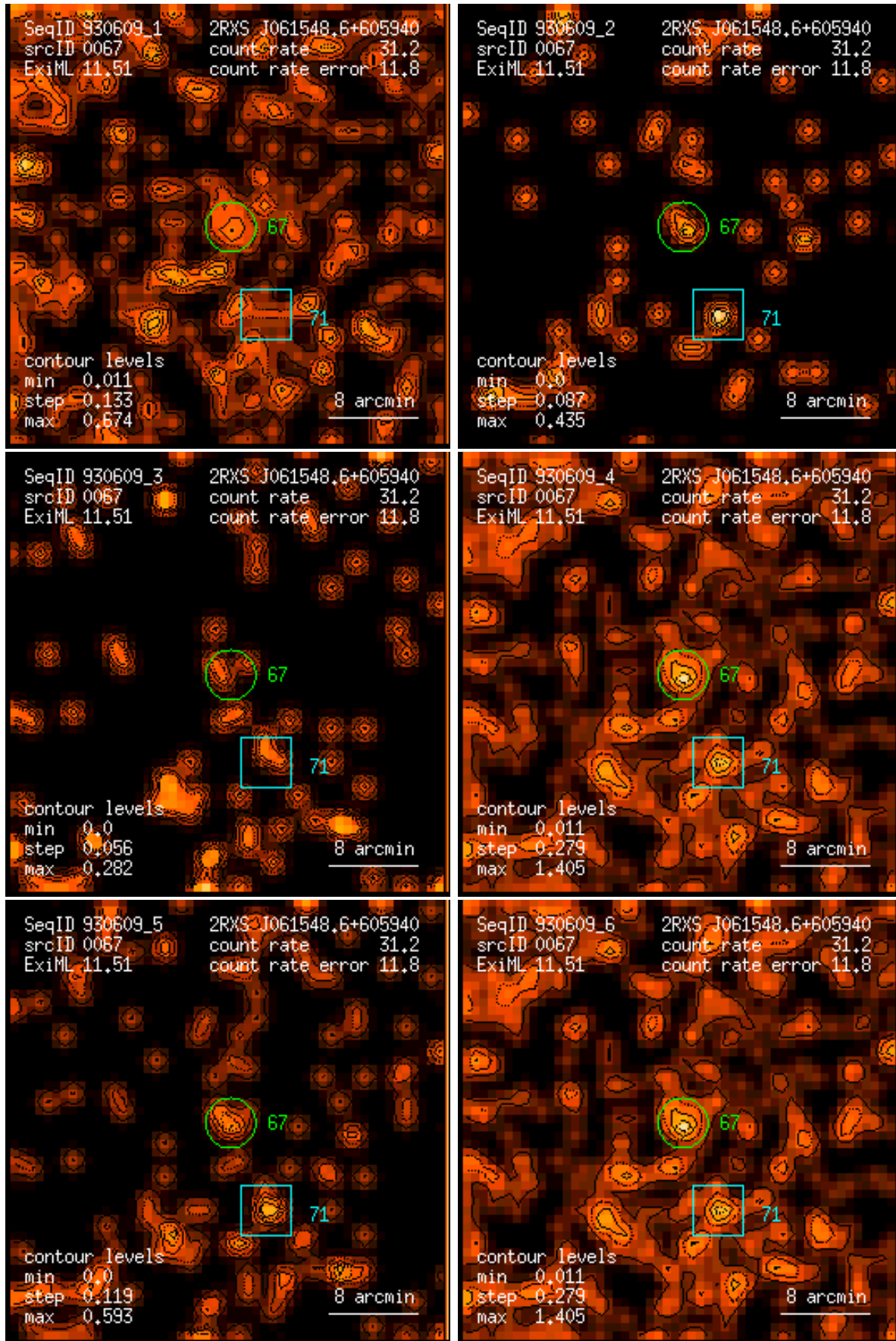
Figure 67: RASS 930609: detection 0067: band rate images, Gaussian filter: (1) PSPC channels 11 – 41, (2) 52 – 90, (3) 91 – 201, (4) 11 – 235, (5) 52 – 201, (6) 11 – 201. Broad band rates in counts/ks. Band rate contour levels in counts/ks/arcmin 2 .
