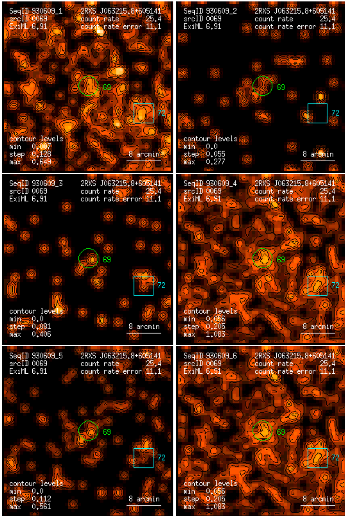
Figure 69: RASS 930609: detection 0069: band rate images, Gaussian filter: (1) PSPC channels 11 – 41, (2) 52 – 90, (3) 91 – 201, (4) 11 – 235, (5) 52 – 201, (6) 11 – 201. Broad band rates in counts/ks. Band rate contour levels in counts/ks/arcmin 2 .
