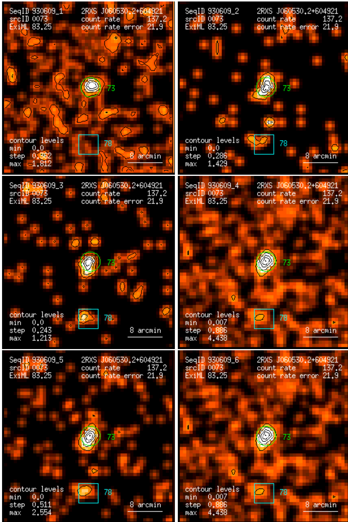
Figure 73: RASS 930609: detection 0073: band rate images, Gaussian filter: (1) PSPC channels 11 – 41, (2) 52 – 90, (3) 91 – 201, (4) 11 – 235, (5) 52 – 201, (6) 11 – 201. Broad band rates in counts/ks. Band rate contour levels in counts/ks/arcmin 2 .
