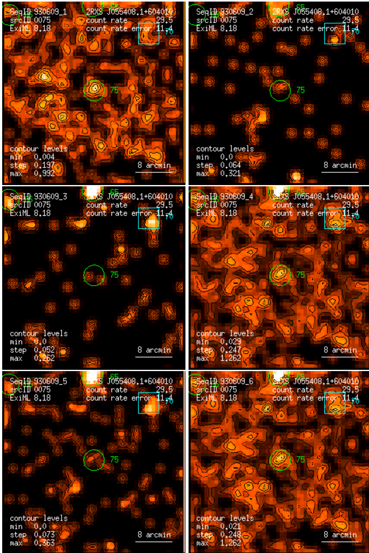
Figure 75: RASS 930609: detection 0075: band rate images, Gaussian filter: (1) PSPC channels 11 – 41, (2) 52 – 90, (3) 91 – 201, (4) 11 – 235, (5) 52 – 201, (6) 11 – 201. Broad band rates in counts/ks. Band rate contour levels in counts/ks/arcmin 2 .
