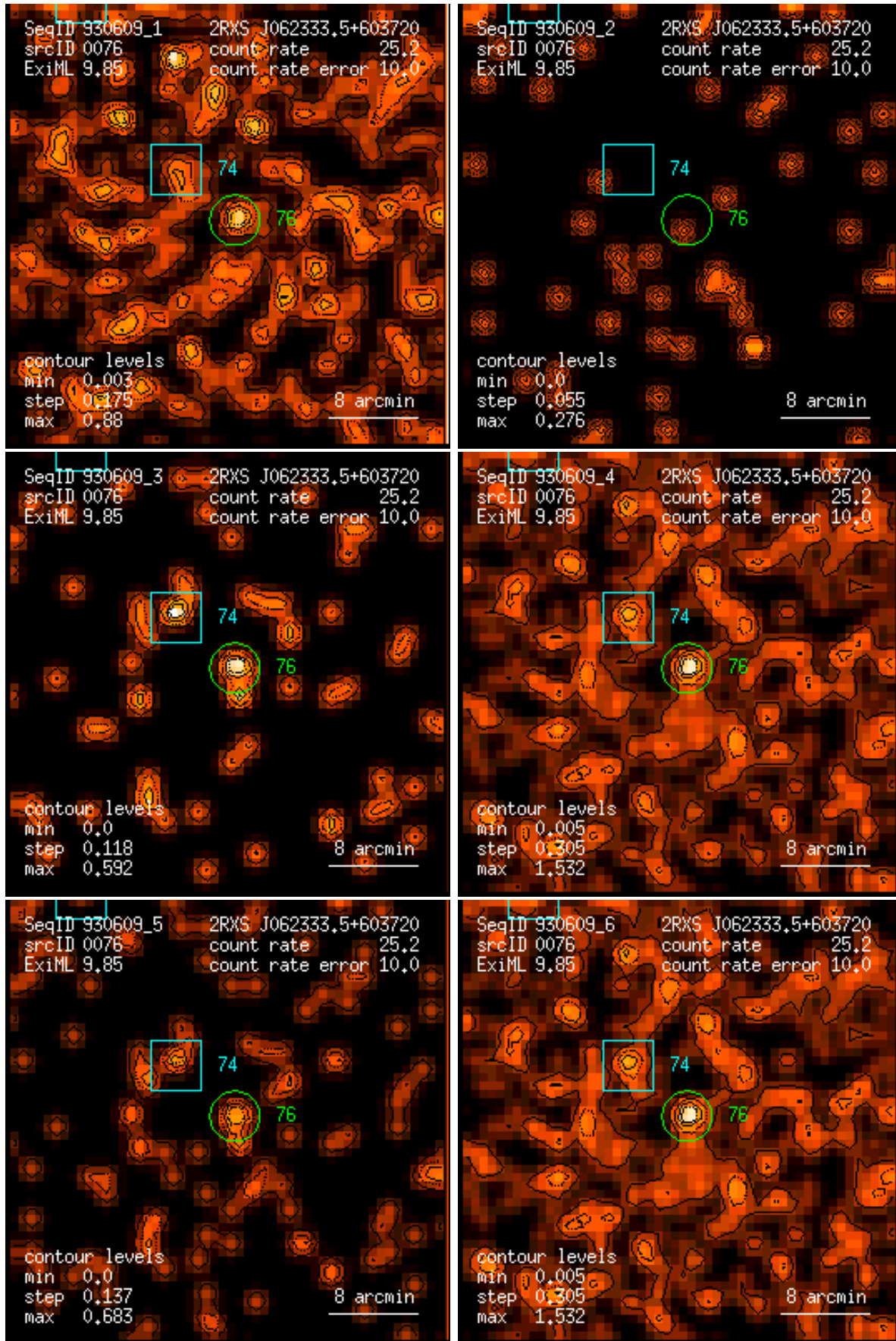
Figure 76: RASS 930609: detection 0076: band rate images, Gaussian filter: (1) PSPC channels 11 – 41, (2) 52 – 90, (3) 91 – 201, (4) 11 – 235, (5) 52 – 201, (6) 11 – 201. Broad band rates in counts/ks. Band rate contour levels in counts/ks/arcmin 2 .
