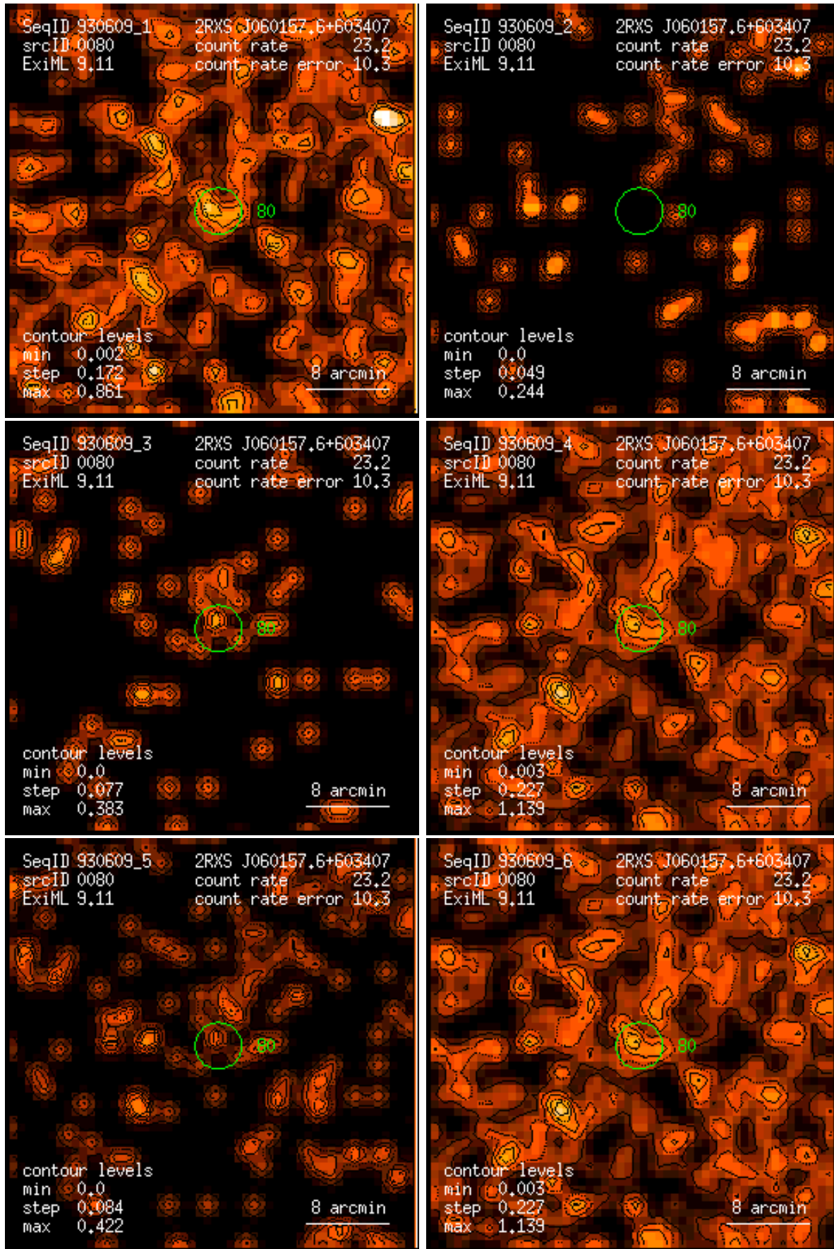
Figure 80: RASS 930609: detection 0080: band rate images, Gaussian filter: (1) PSPC channels 11 – 41, (2) 52 – 90, (3) 91 – 201, (4) 11 – 235, (5) 52 – 201, (6) 11 – 201. Broad band rates in counts/ks. Band rate contour levels in counts/ks/arcmin 2 .
