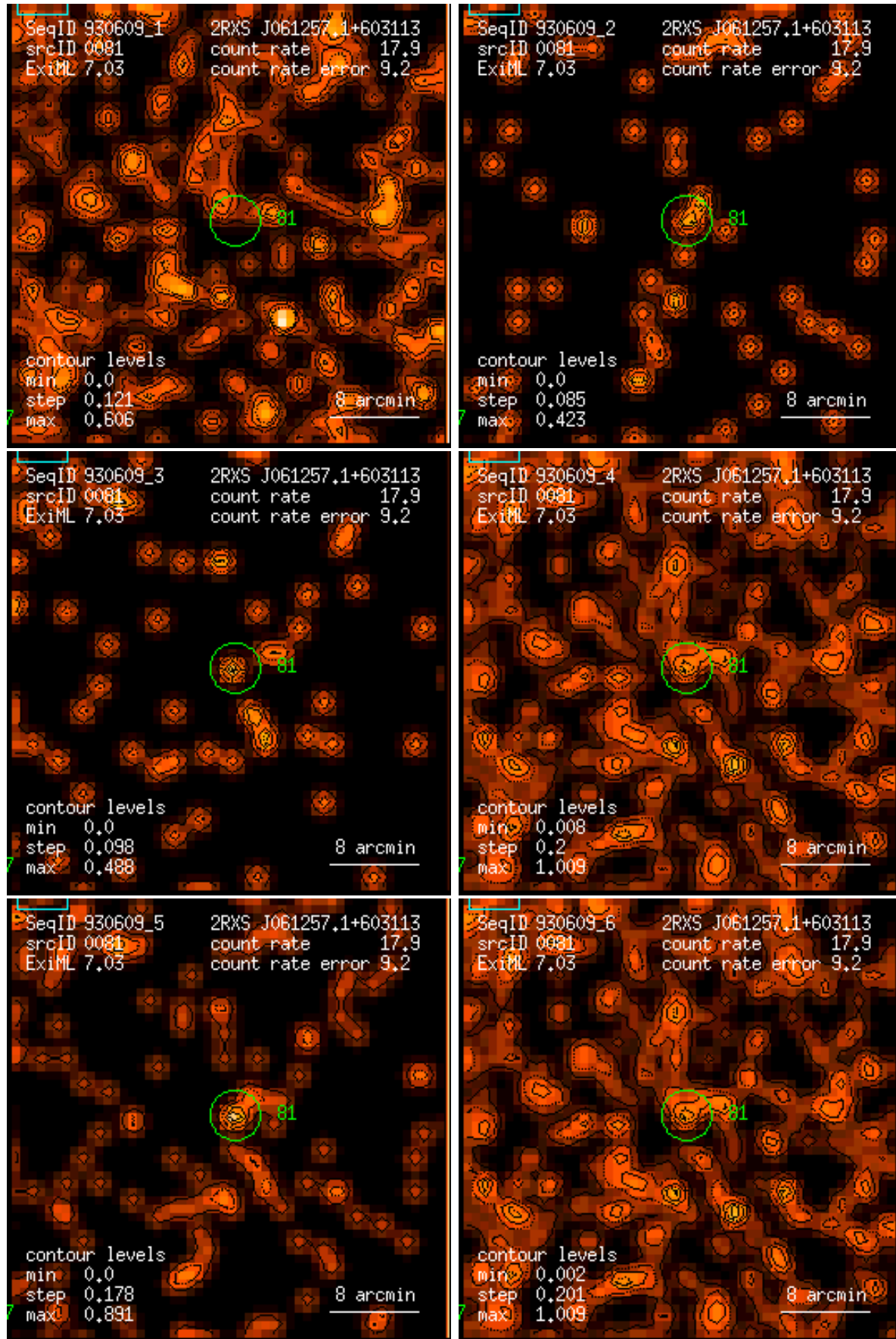
Figure 81: RASS 930609: detection 0081: band rate images, Gaussian filter: (1) PSPC channels 11 – 41, (2) 52 – 90, (3) 91 – 201, (4) 11 – 235, (5) 52 – 201, (6) 11 – 201. Broad band rates in counts/ks. Band rate contour levels in counts/ks/arcmin 2 .
