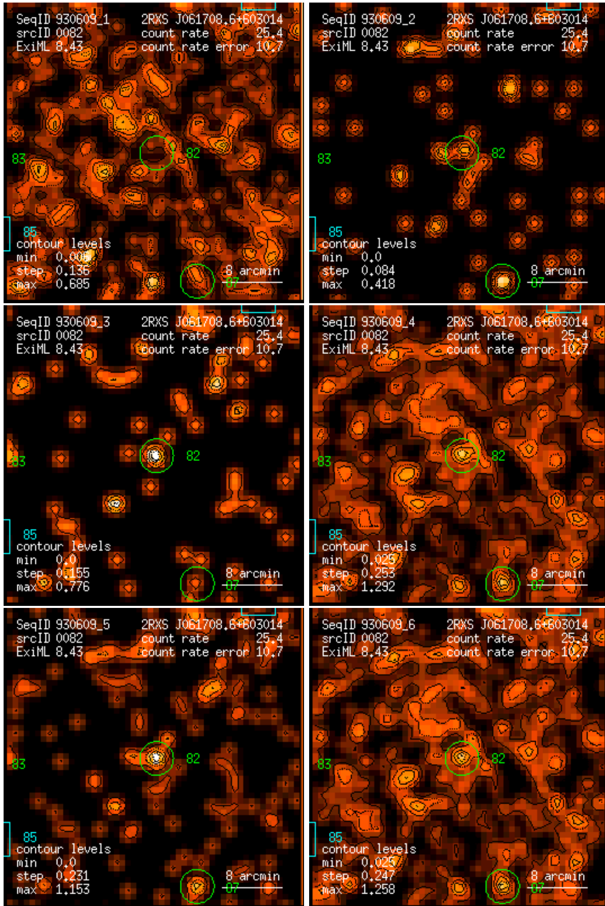
Figure 82: RASS 930609: detection 0082: band rate images, Gaussian filter: (1) PSPC channels 11 – 41, (2) 52 – 90, (3) 91 – 201, (4) 11 – 235, (5) 52 – 201, (6) 11 – 201. Broad band rates in counts/ks. Band rate contour levels in counts/ks/arcmin 2 .
