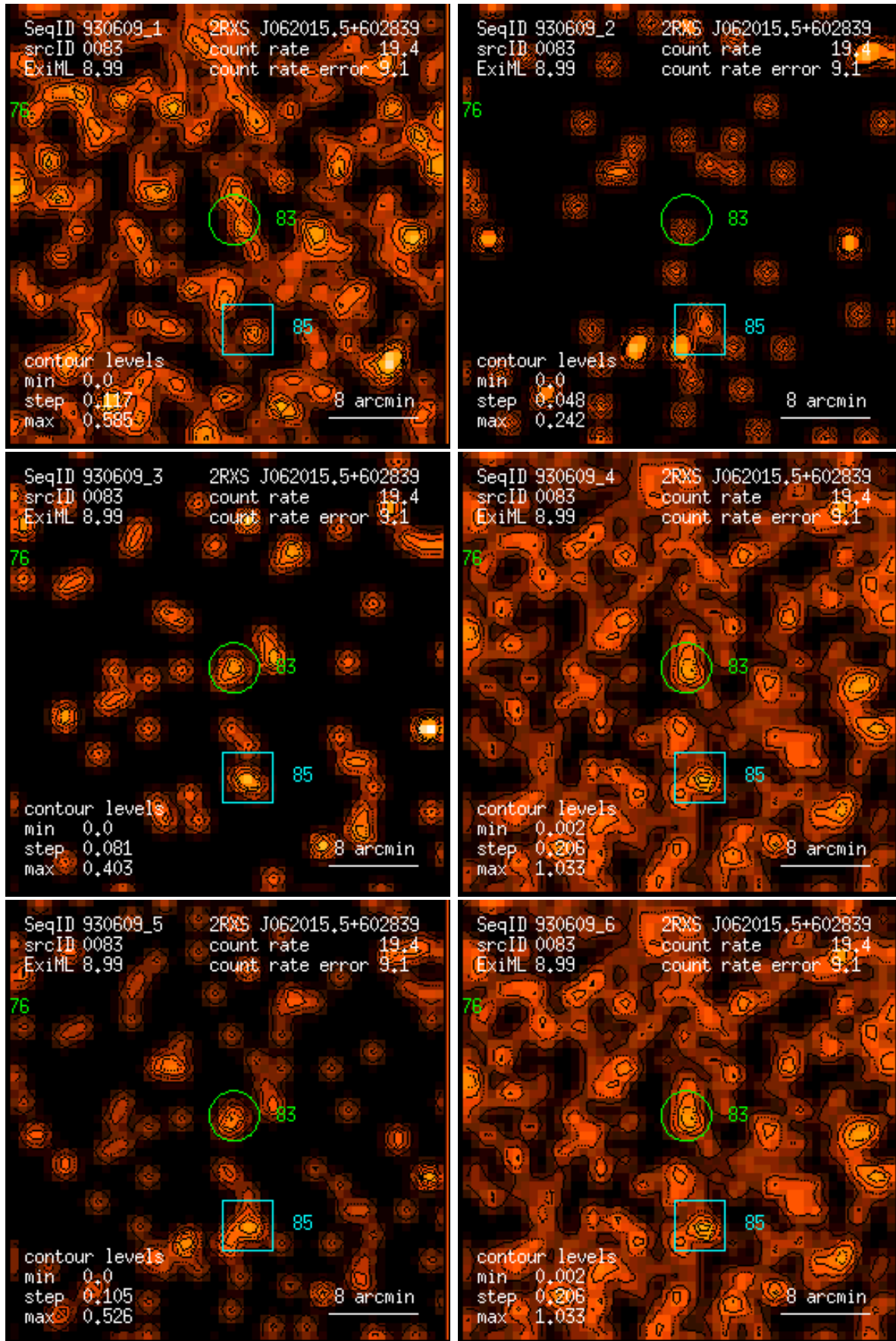
Figure 83: RASS 930609: detection 0083: band rate images, Gaussian filter: (1) PSPC channels 11 – 41, (2) 52 – 90, (3) 91 – 201, (4) 11 – 235, (5) 52 – 201, (6) 11 – 201. Broad band rates in counts/ks. Band rate contour levels in counts/ks/arcmin 2 .
