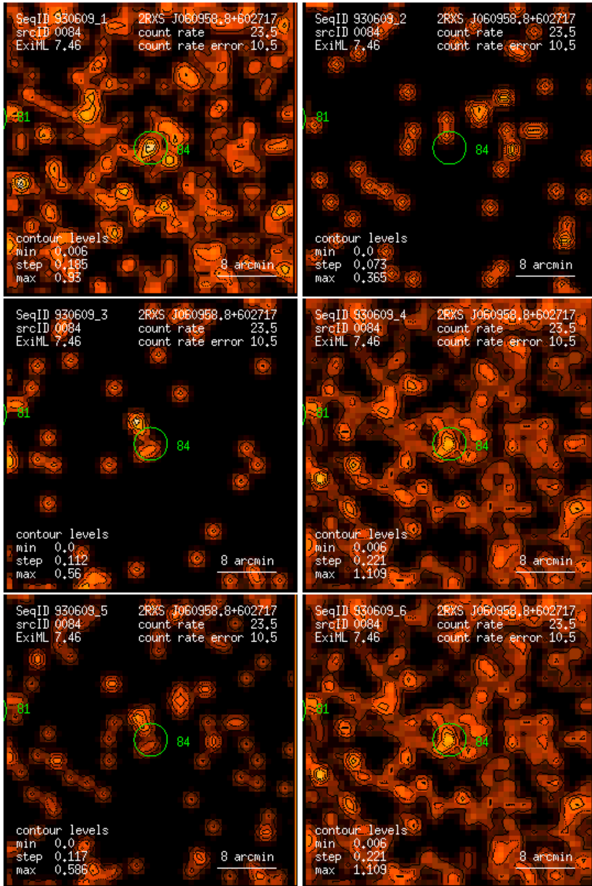
Figure 84: RASS 930609: detection 0084: band rate images, Gaussian filter: (1) PSPC channels 11 – 41, (2) 52 – 90, (3) 91 – 201, (4) 11 – 235, (5) 52 – 201, (6) 11 – 201. Broad band rates in counts/ks. Band rate contour levels in counts/ks/arcmin 2 .
