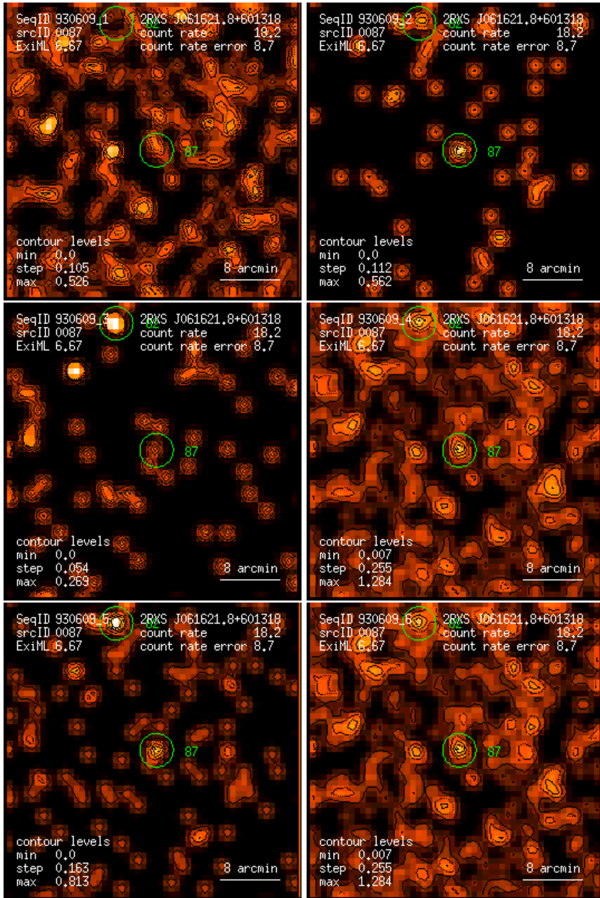
Figure 87: RASS 930609: detection 0087: band rate images, Gaussian filter: (1) PSPC channels 11 – 41, (2) 52 – 90, (3) 91 – 201, (4) 11 – 235, (5) 52 – 201, (6) 11 – 201. Broad band rates in counts/ks. Band rate contour levels in counts/ks/arcmin 2 .
