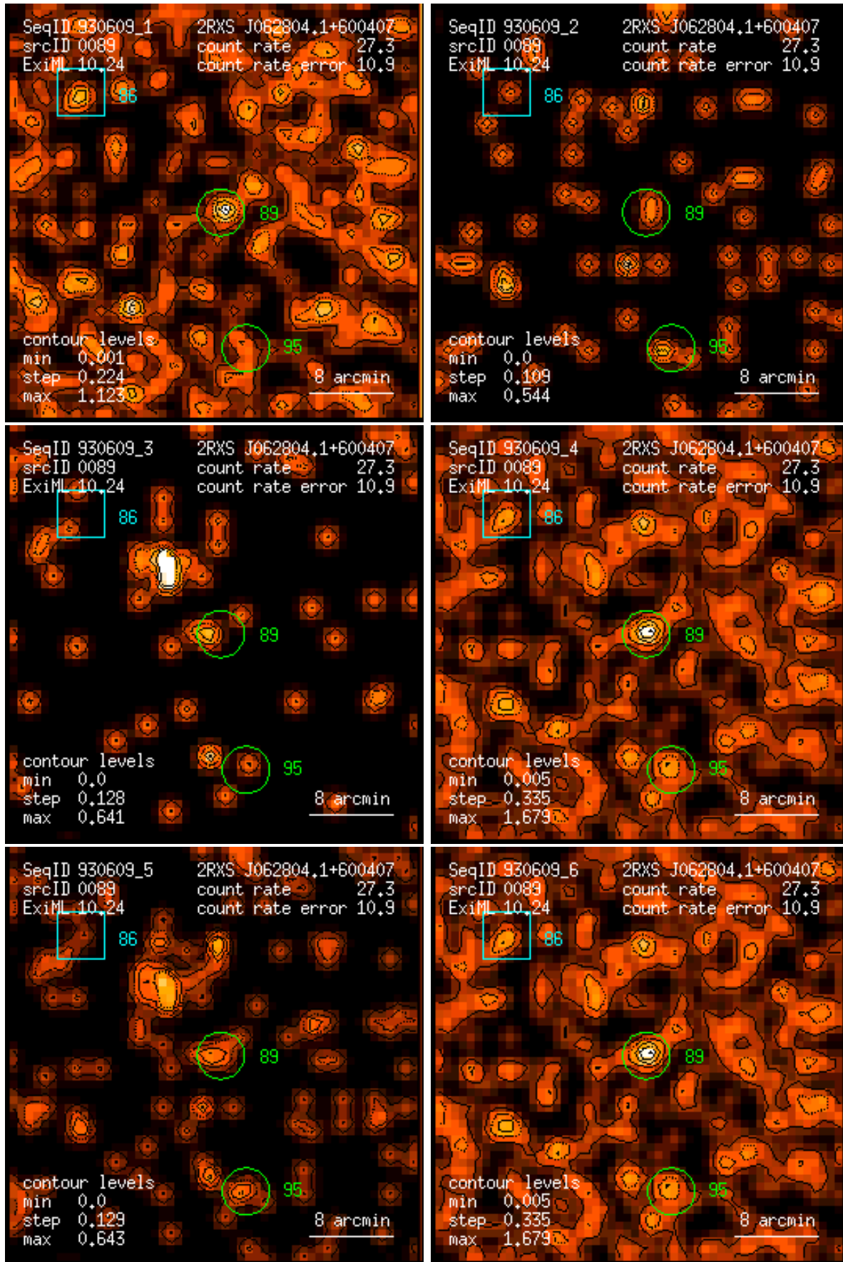
Figure 89: RASS 930609: detection 0089: band rate images, Gaussian filter: (1) PSPC channels 11 – 41, (2) 52 – 90, (3) 91 – 201, (4) 11 – 235, (5) 52 – 201, (6) 11 – 201. Broad band rates in counts/ks. Band rate contour levels in counts/ks/arcmin 2 .
