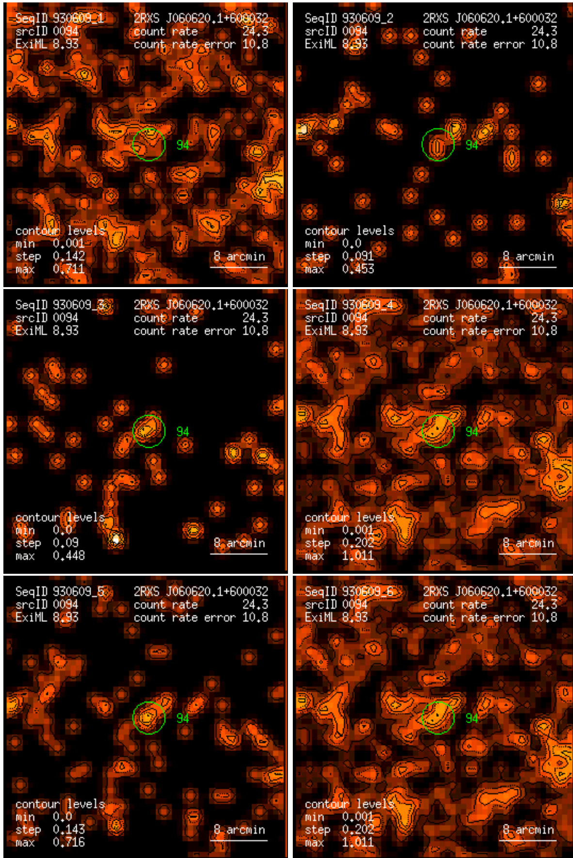
Figure 94: RASS 930609: detection 0094: band rate images, Gaussian filter: (1) PSPC channels 11 – 41, (2) 52 – 90, (3) 91 – 201, (4) 11 – 235, (5) 52 – 201, (6) 11 – 201. Broad band rates in counts/ks. Band rate contour levels in counts/ks/arcmin 2 .
