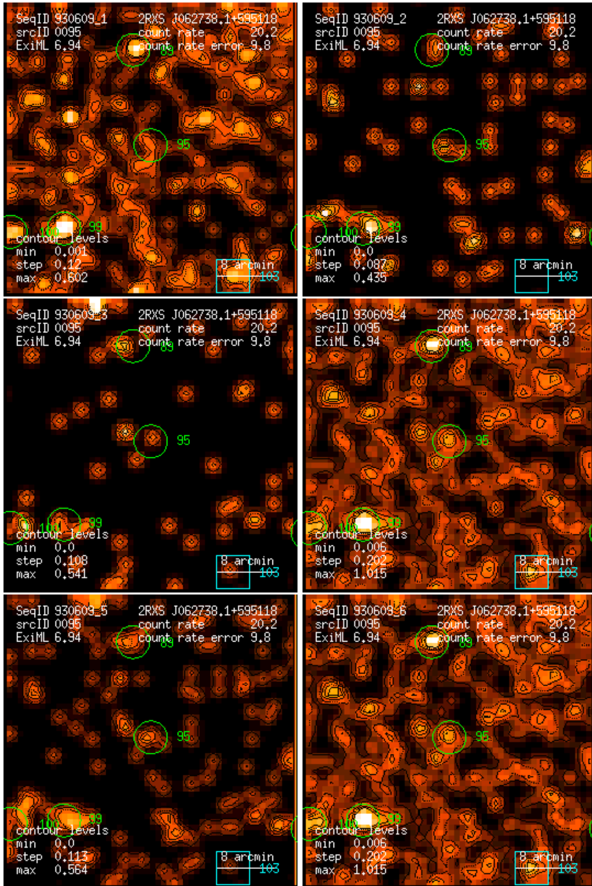
Figure 95: RASS 930609: detection 0095: band rate images, Gaussian filter: (1) PSPC channels 11 – 41, (2) 52 – 90, (3) 91 – 201, (4) 11 – 235, (5) 52 – 201, (6) 11 – 201. Broad band rates in counts/ks. Band rate contour levels in counts/ks/arcmin 2 .
