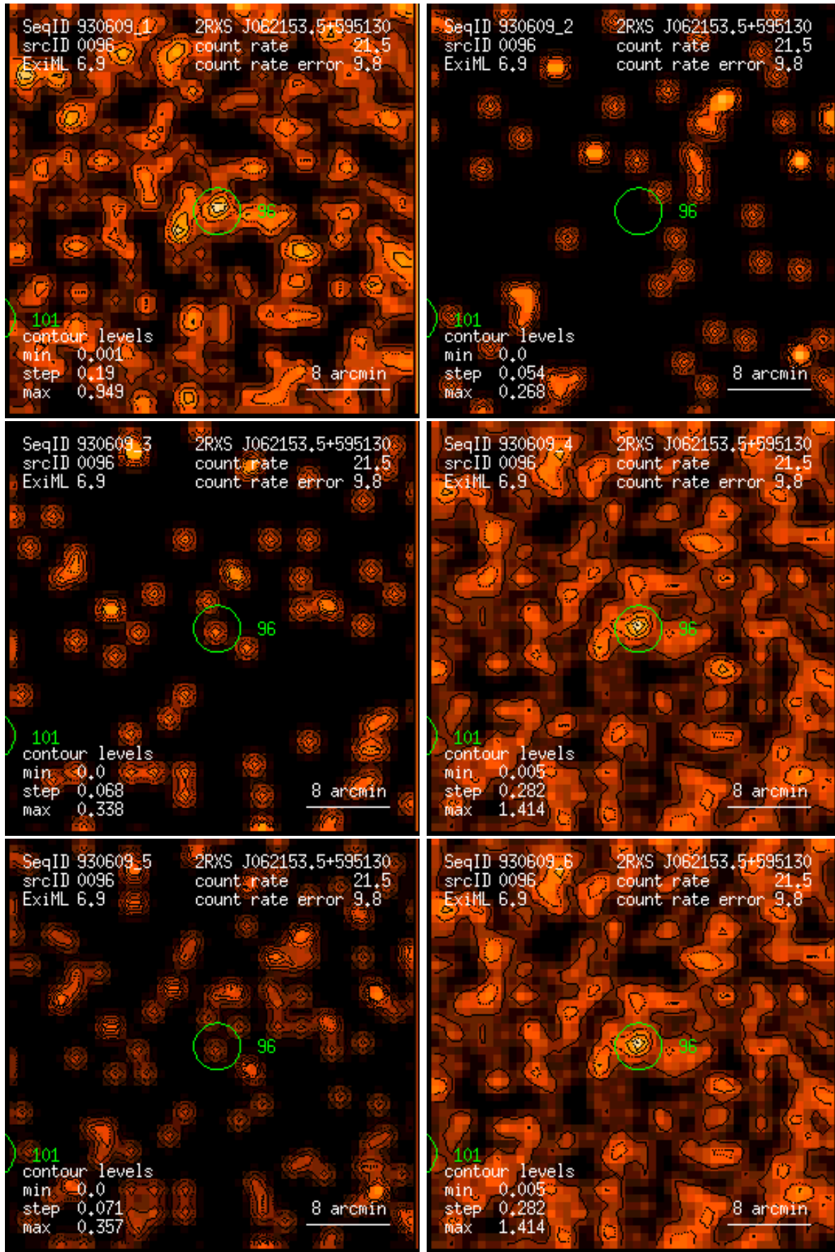
Figure 96: RASS 930609: detection 0096: band rate images, Gaussian filter: (1) PSPC channels 11 – 41, (2) 52 – 90, (3) 91 – 201, (4) 11 – 235, (5) 52 – 201, (6) 11 – 201. Broad band rates in counts/ks. Band rate contour levels in counts/ks/arcmin 2 .
