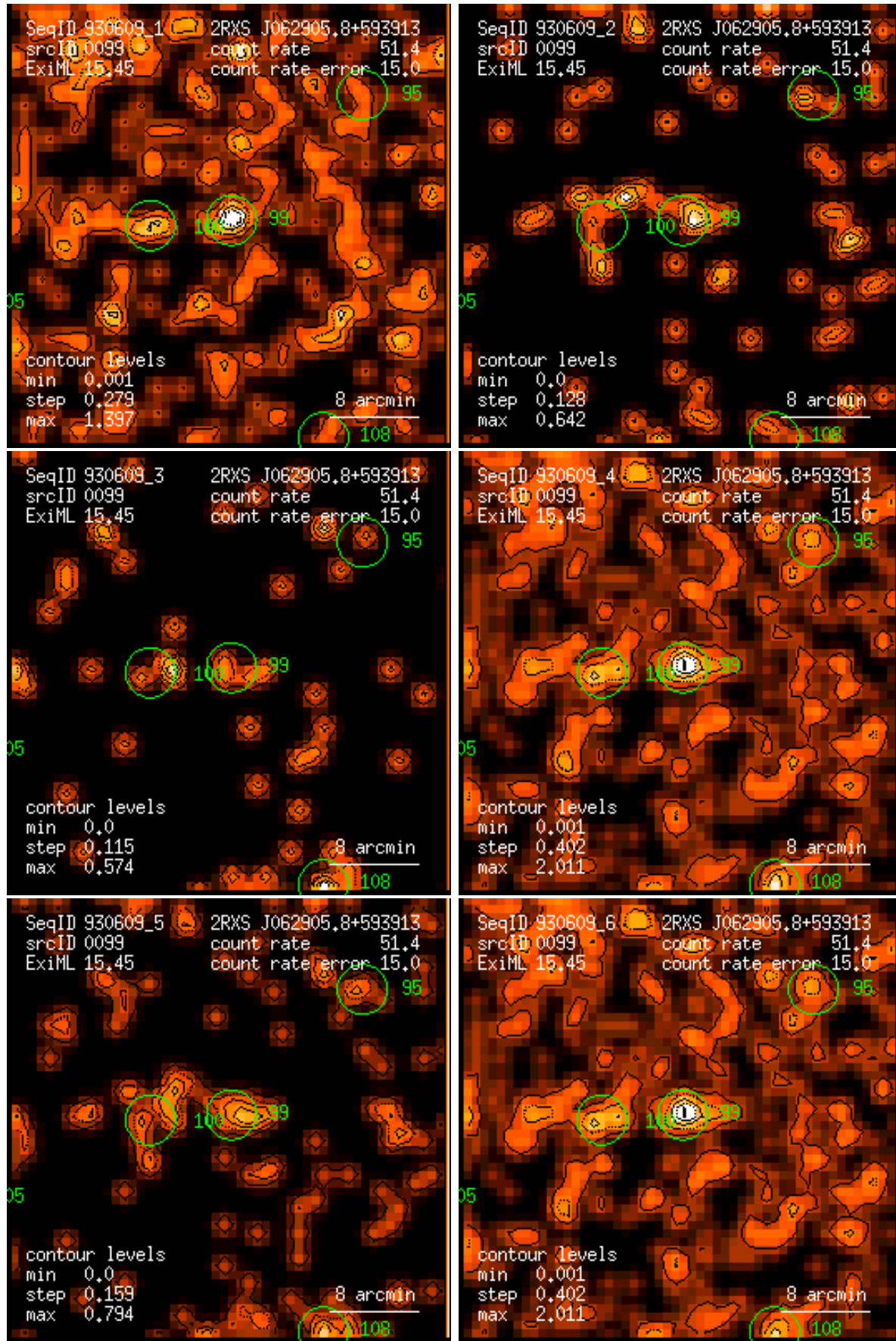
Figure 99: RASS 930609: detection 0099: band rate images, Gaussian filter: (1) PSPC channels 11 – 41, (2) 52 – 90, (3) 91 – 201, (4) 11 – 235, (5) 52 – 201, (6) 11 – 201. Broad band rates in counts/ks. Band rate contour levels in counts/ks/arcmin 2 .
