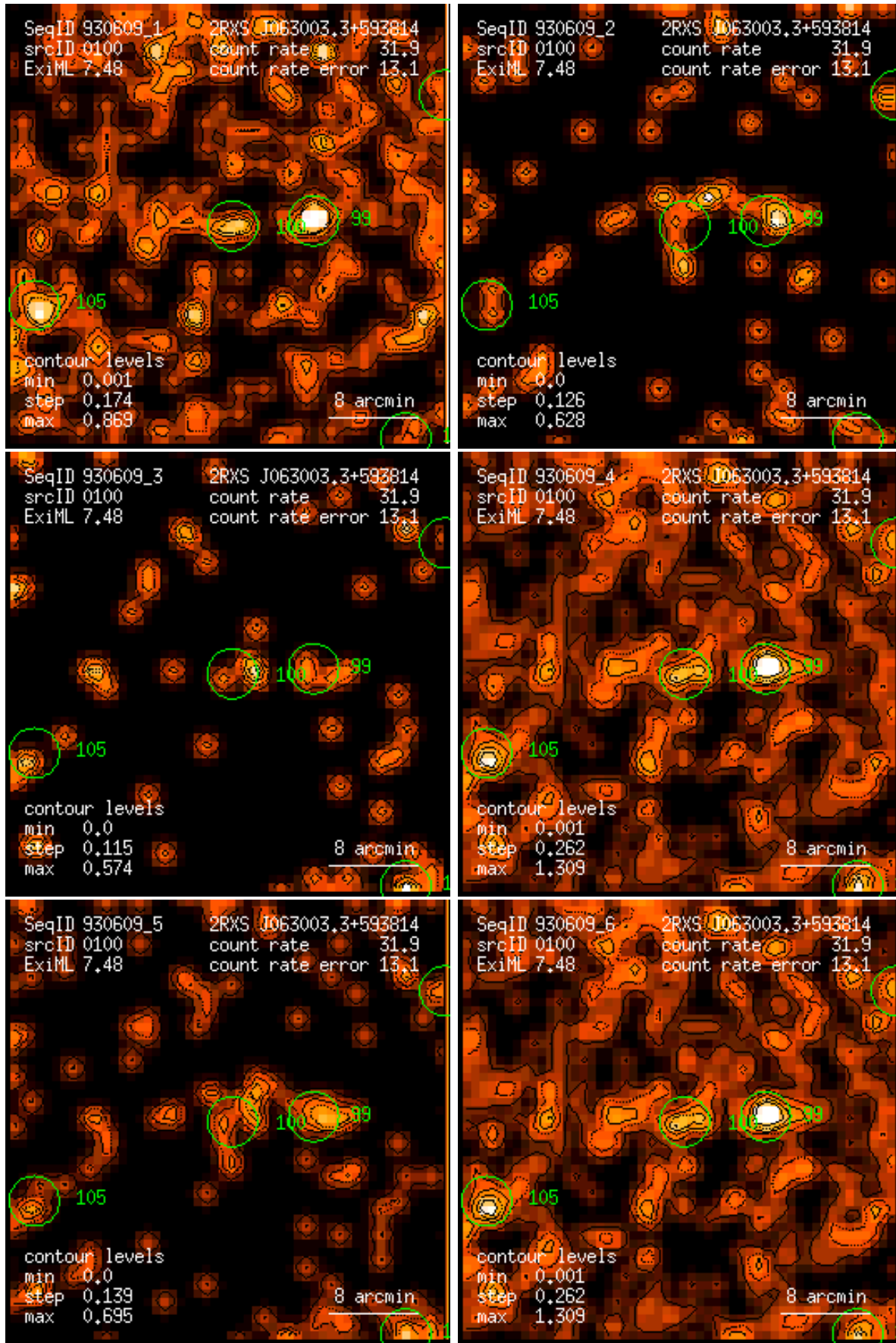
Figure 100: RASS 930609: detection 0100: band rate images, Gaussian filter: (1) PSPC channels 11 – 41, (2) 52 – 90, (3) 91 – 201, (4) 11 – 235, (5) 52 – 201, (6) 11 – 201. Broad band rates in counts/ks. Band rate contour levels in counts/ks/arcmin 2 .
