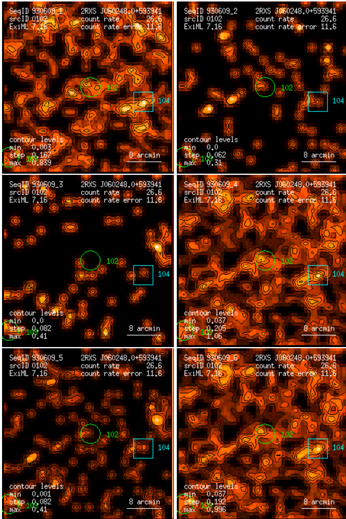
Figure 102: RASS 930609: detection 0102: band rate images, Gaussian filter: (1) PSPC channels 11 – 41, (2) 52 – 90, (3) 91 – 201, (4) 11 – 235, (5) 52 – 201, (6) 11 – 201. Broad band rates in counts/ks. Band rate contour levels in counts/ks/arcmin 2 .
