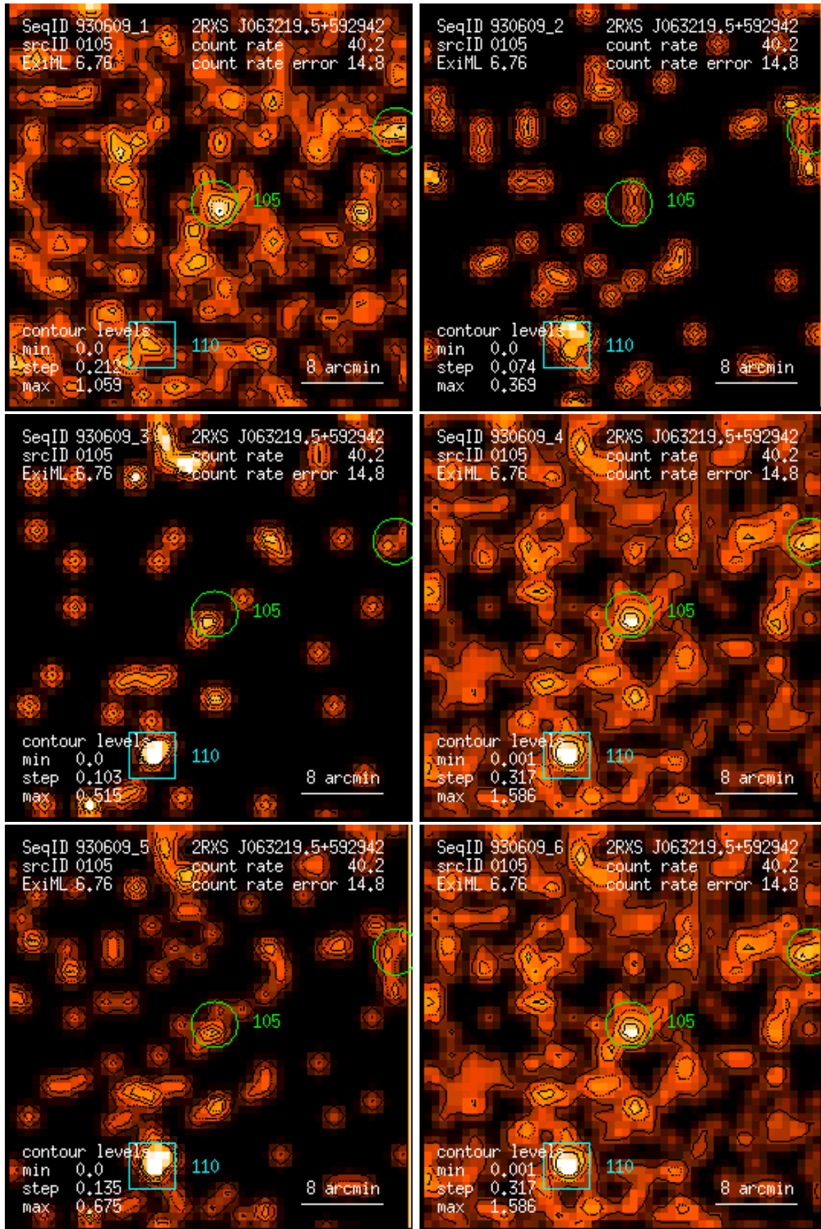
Figure 105: RASS 930609: detection 0105: band rate images, Gaussian filter: (1) PSPC channels 11 – 41, (2) 52 – 90, (3) 91 – 201, (4) 11 – 235, (5) 52 – 201, (6) 11 – 201. Broad band rates in counts/ks. Band rate contour levels in counts/ks/arcmin 2 .
