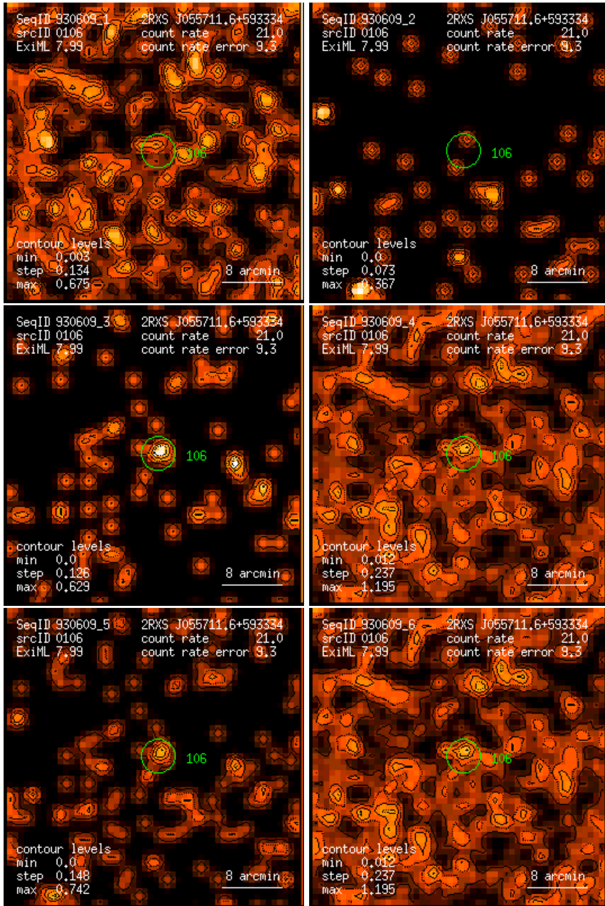
Figure 106: RASS 930609: detection 0106: band rate images, Gaussian filter: (1) PSPC channels 11 – 41, (2) 52 – 90, (3) 91 – 201, (4) 11 – 235, (5) 52 – 201, (6) 11 – 201. Broad band rates in counts/ks. Band rate contour levels in counts/ks/arcmin 2 .
