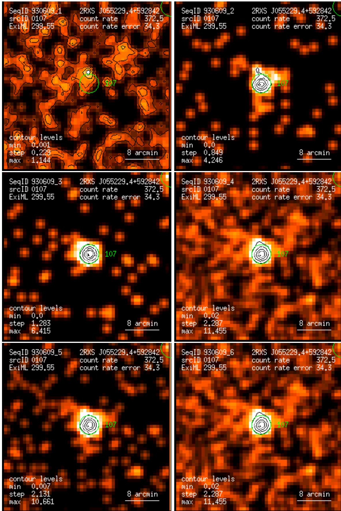
Figure 107: RASS 930609: detection 0107: band rate images, Gaussian filter: (1) PSPC channels 11 – 41, (2) 52 – 90, (3) 91 – 201, (4) 11 – 235, (5) 52 – 201, (6) 11 – 201. Broad band rates in counts/ks. Band rate contour levels in counts/ks/arcmin 2 .
