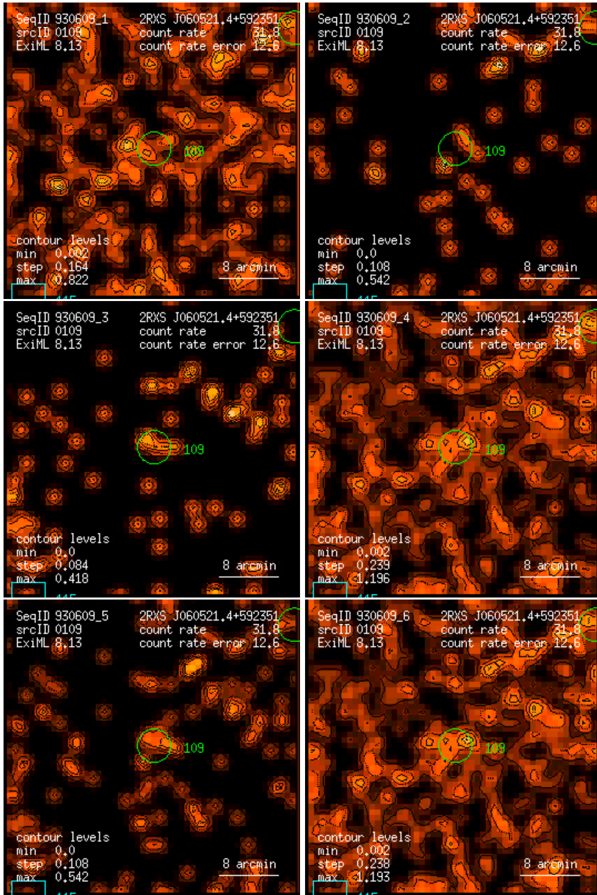
Figure 109: RASS 930609: detection 0109: band rate images, Gaussian filter: (1) PSPC channels 11 – 41, (2) 52 – 90, (3) 91 – 201, (4) 11 – 235, (5) 52 – 201, (6) 11 – 201. Broad band rates in counts/ks. Band rate contour levels in counts/ks/arcmin 2 .
