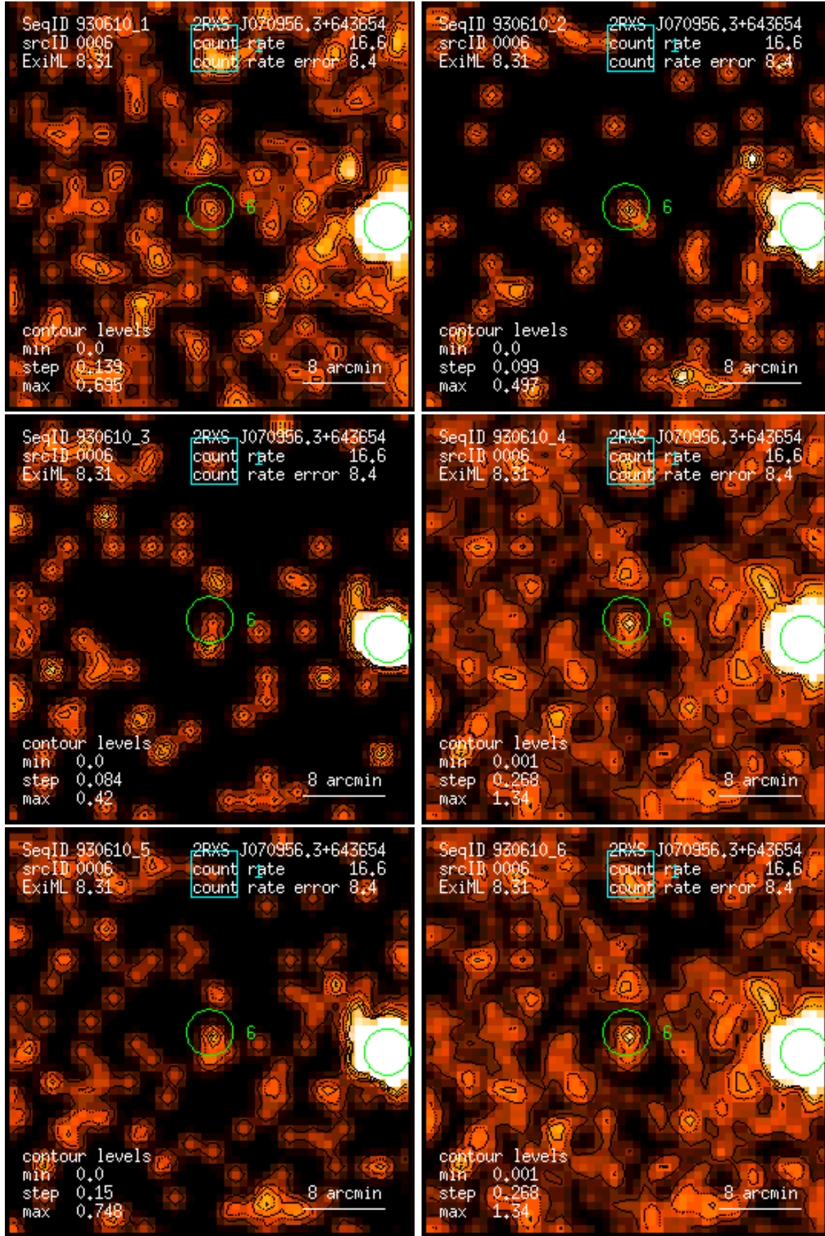
Figure 6: RASS 930610: detection 0006: band rate images, Gaussian filter: (1) PSPC channels 11 – 41, (2) 52 – 90, (3) 91 – 201, (4) 11 – 235, (5) 52 – 201, (6) 11 – 201. Broad band rates in counts/ks. Band rate contour levels in counts/ks/arcmin 2 .
