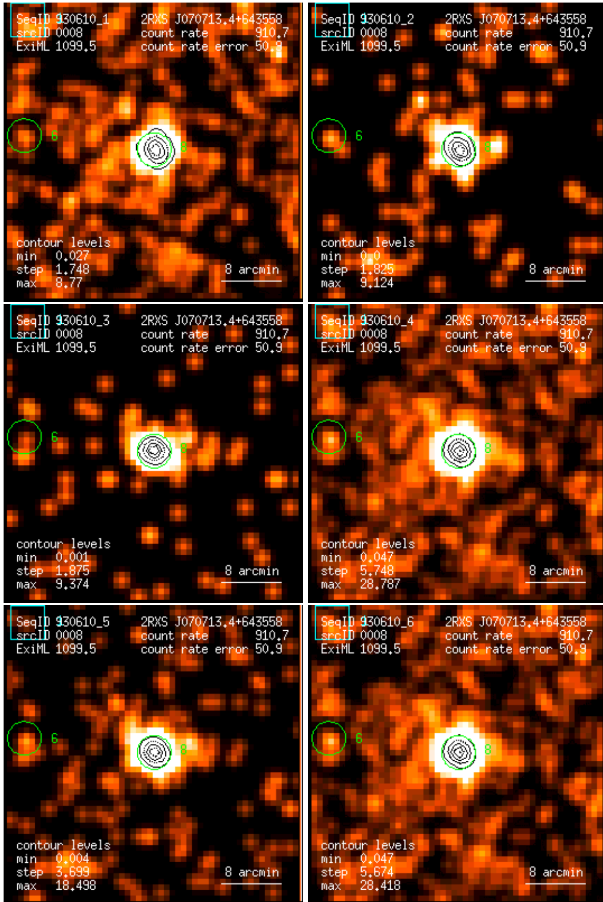
Figure 8: RASS 930610: detection 0008: band rate images, Gaussian filter: (1) PSPC channels 11 – 41, (2) 52 – 90, (3) 91 – 201, (4) 11 – 235, (5) 52 – 201, (6) 11 – 201. Broad band rates in counts/ks. Band rate contour levels in counts/ks/arcmin 2 .
