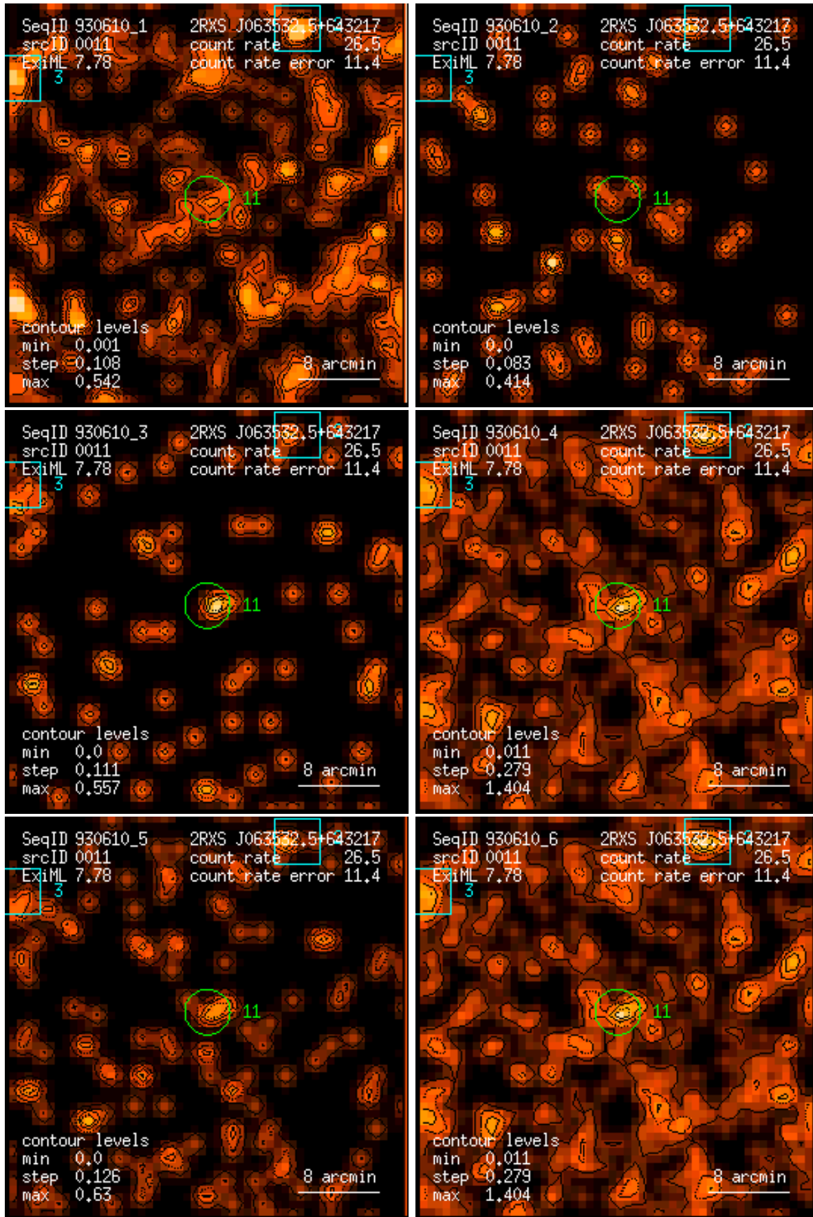
Figure 11: RASS 930610: detection 0011: band rate images, Gaussian filter: (1) PSPC channels 11 – 41, (2) 52 – 90, (3) 91 – 201, (4) 11 – 235, (5) 52 – 201, (6) 11 – 201. Broad band rates in counts/ks. Band rate contour levels in counts/ks/arcmin 2 .
