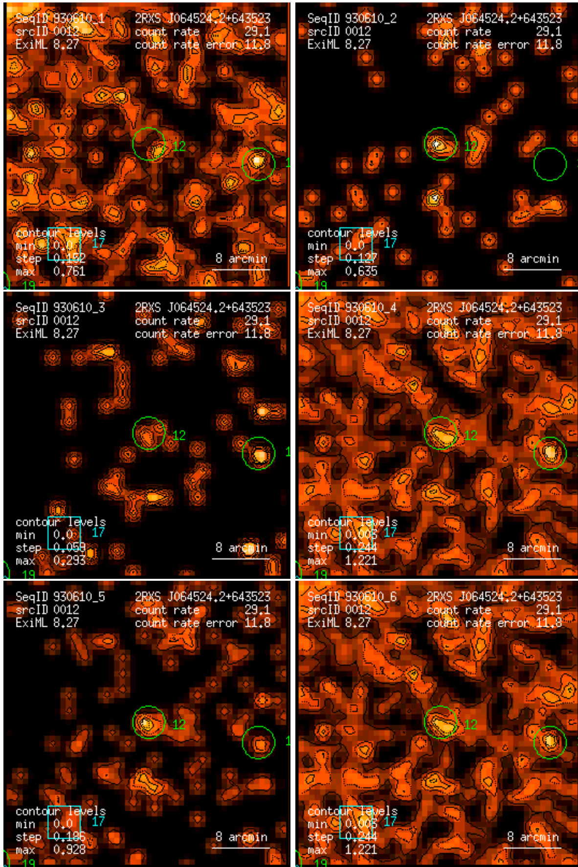
Figure 12: RASS 930610: detection 0012: band rate images, Gaussian filter: (1) PSPC channels 11 – 41, (2) 52 – 90, (3) 91 – 201, (4) 11 – 235, (5) 52 – 201, (6) 11 – 201. Broad band rates in counts/ks. Band rate contour levels in counts/ks/arcmin 2 .
