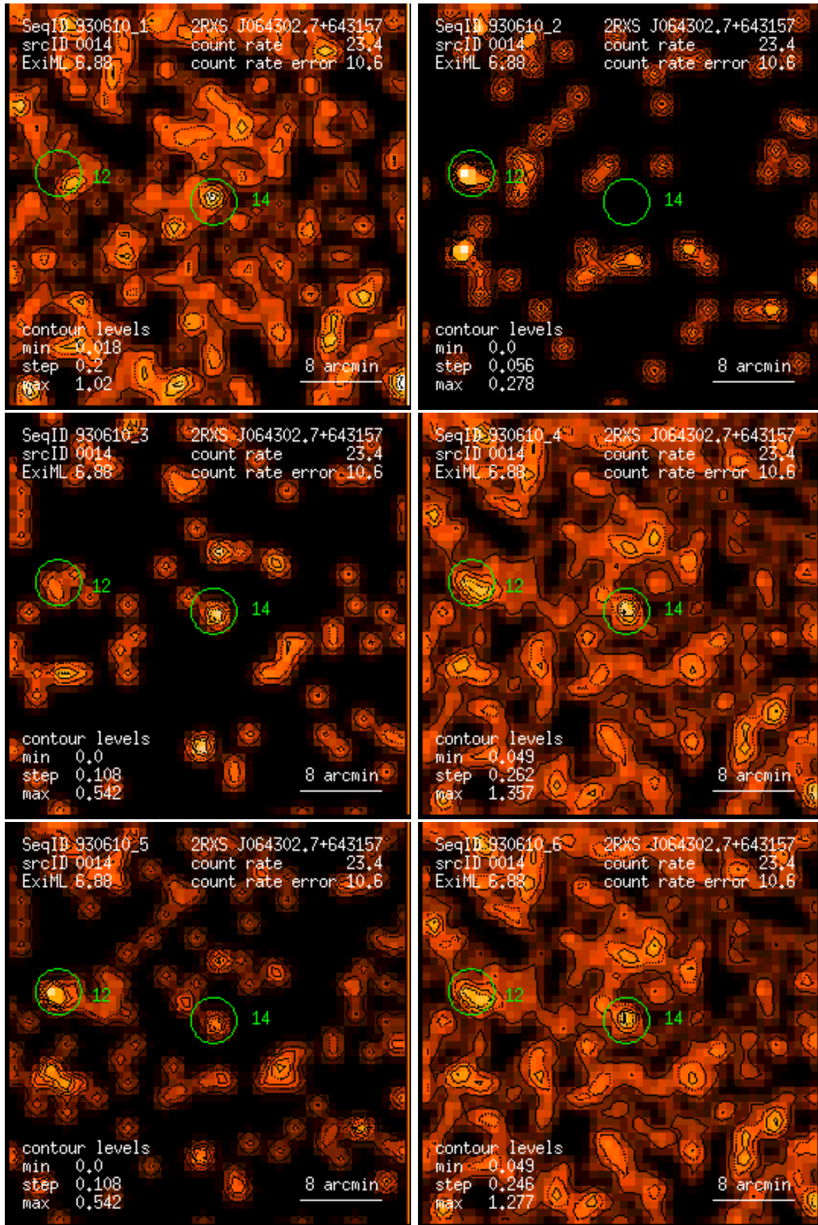
Figure 14: RASS 930610: detection 0014: band rate images, Gaussian filter: (1) PSPC channels 11 – 41, (2) 52 – 90, (3) 91 – 201, (4) 11 – 235, (5) 52 – 201, (6) 11 – 201. Broad band rates in counts/ks. Band rate contour levels in counts/ks/arcmin 2 .
