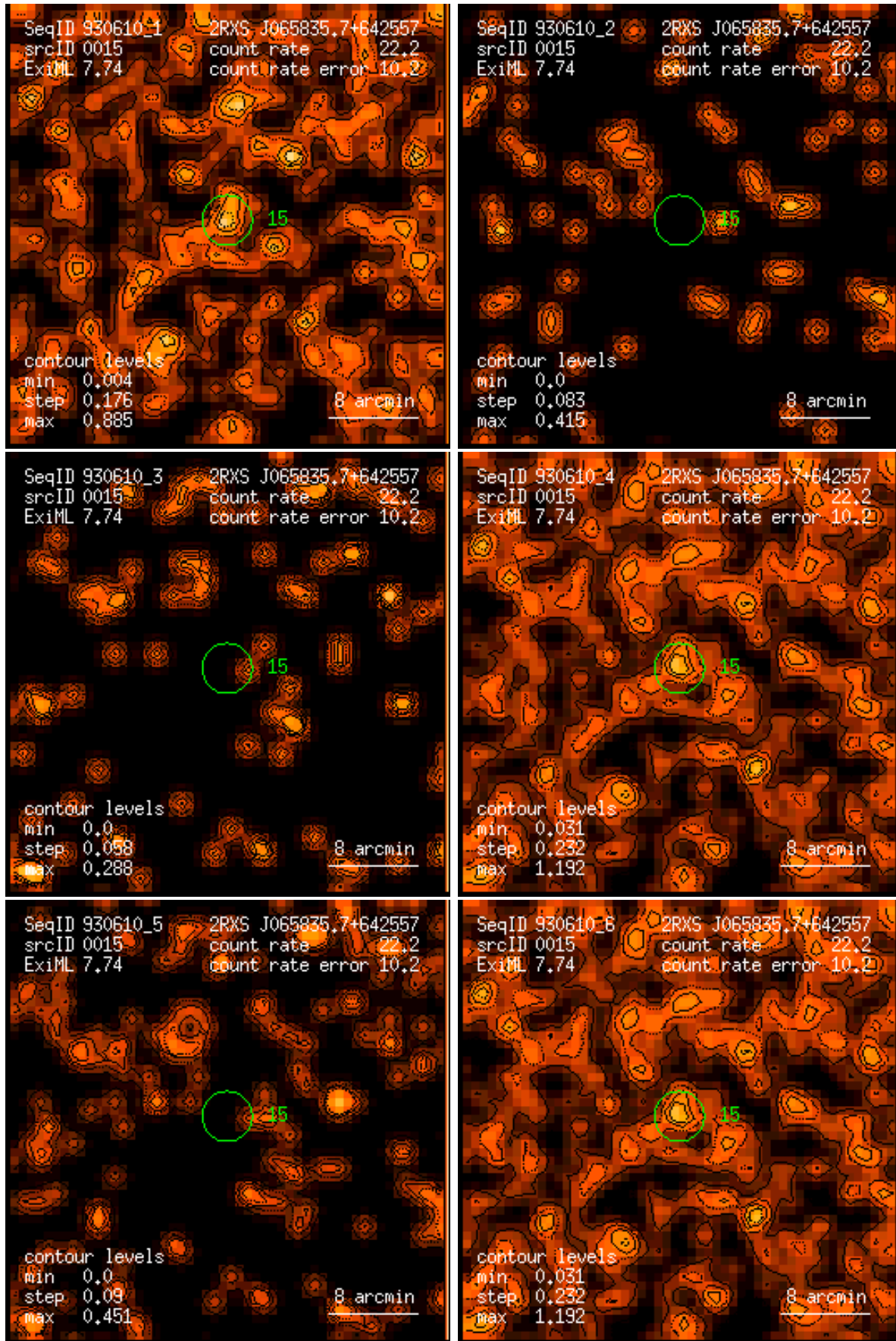
Figure 15: RASS 930610: detection 0015: band rate images, Gaussian filter: (1) PSPC channels 11 – 41, (2) 52 – 90, (3) 91 – 201, (4) 11 – 235, (5) 52 – 201, (6) 11 – 201. Broad band rates in counts/ks. Band rate contour levels in counts/ks/arcmin 2 .
