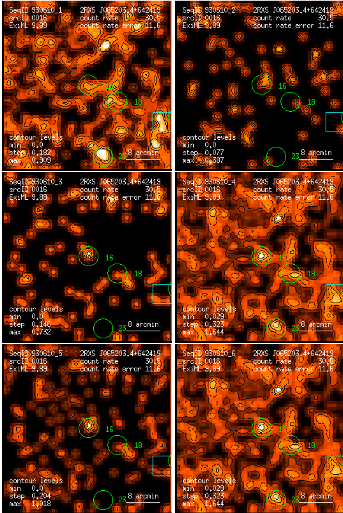
Figure 16: RASS 930610: detection 0016: band rate images, Gaussian filter: (1) PSPC channels 11 – 41, (2) 52 – 90, (3) 91 – 201, (4) 11 – 235, (5) 52 – 201, (6) 11 – 201. Broad band rates in counts/ks. Band rate contour levels in counts/ks/arcmin 2 .
