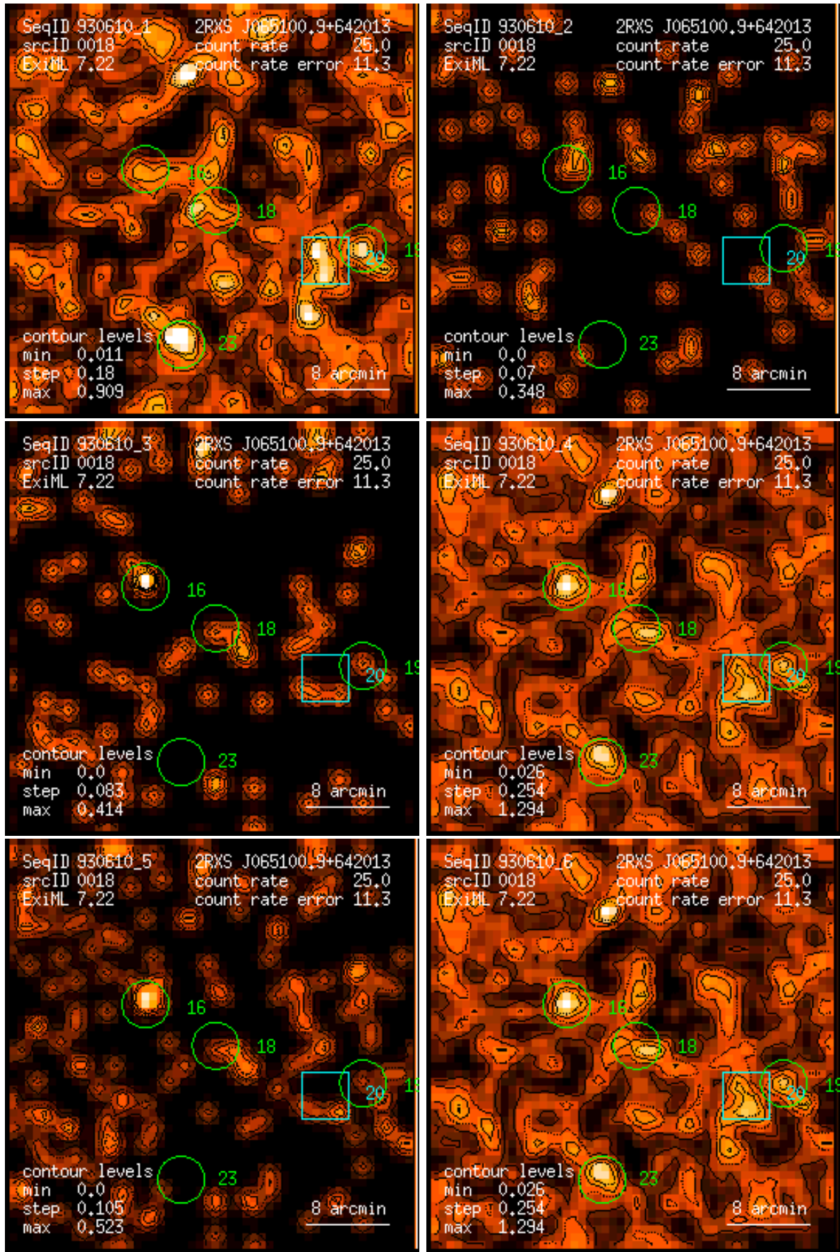
Figure 18: RASS 930610: detection 0018: band rate images, Gaussian filter: (1) PSPC channels 11 – 41, (2) 52 – 90, (3) 91 – 201, (4) 11 – 235, (5) 52 – 201, (6) 11 – 201. Broad band rates in counts/ks. Band rate contour levels in counts/ks/arcmin 2 .
