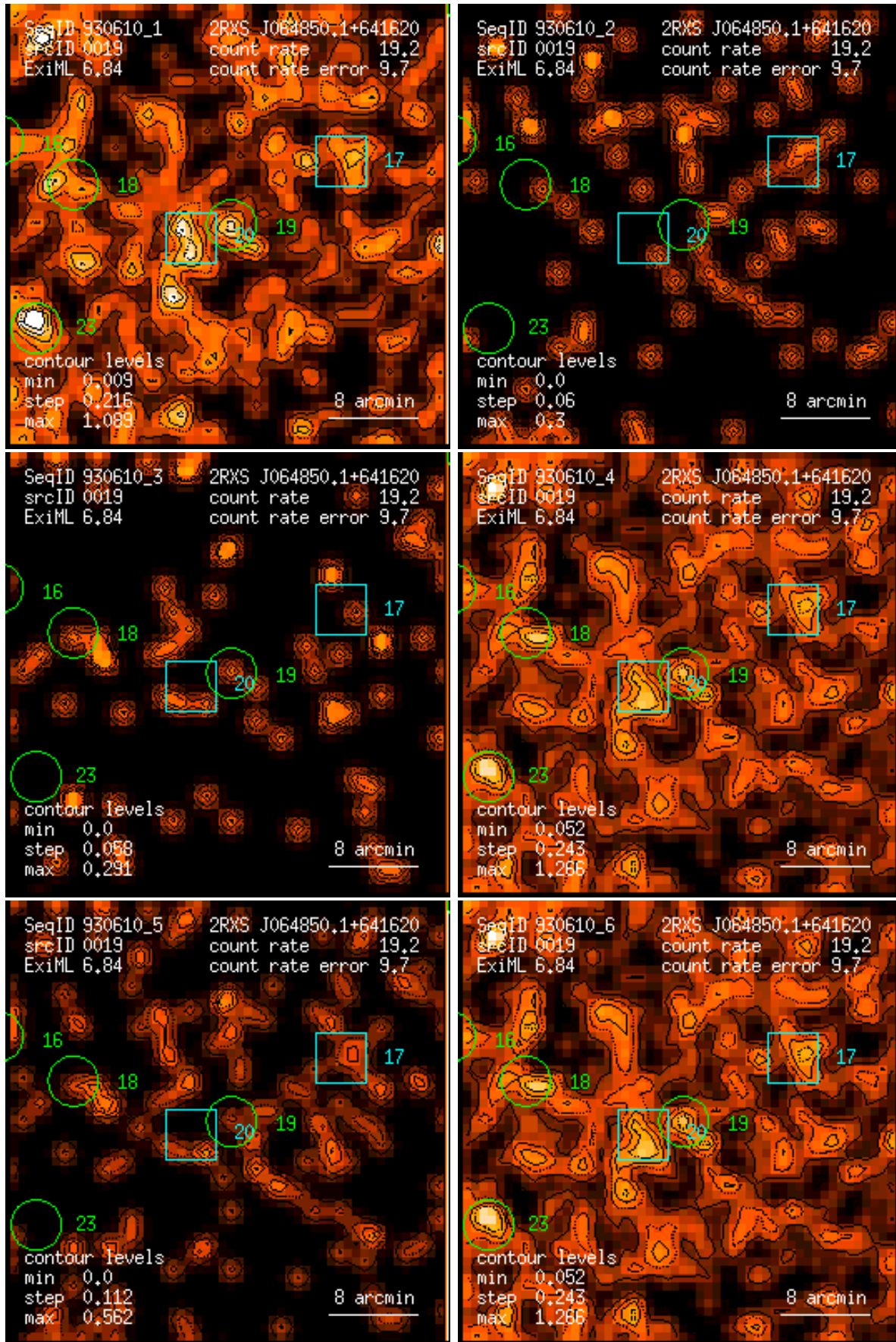
Figure 19: RASS 930610: detection 0019: band rate images, Gaussian filter: (1) PSPC channels 11 – 41, (2) 52 – 90, (3) 91 – 201, (4) 11 – 235, (5) 52 – 201, (6) 11 – 201. Broad band rates in counts/ks. Band rate contour levels in counts/ks/arcmin 2 .
