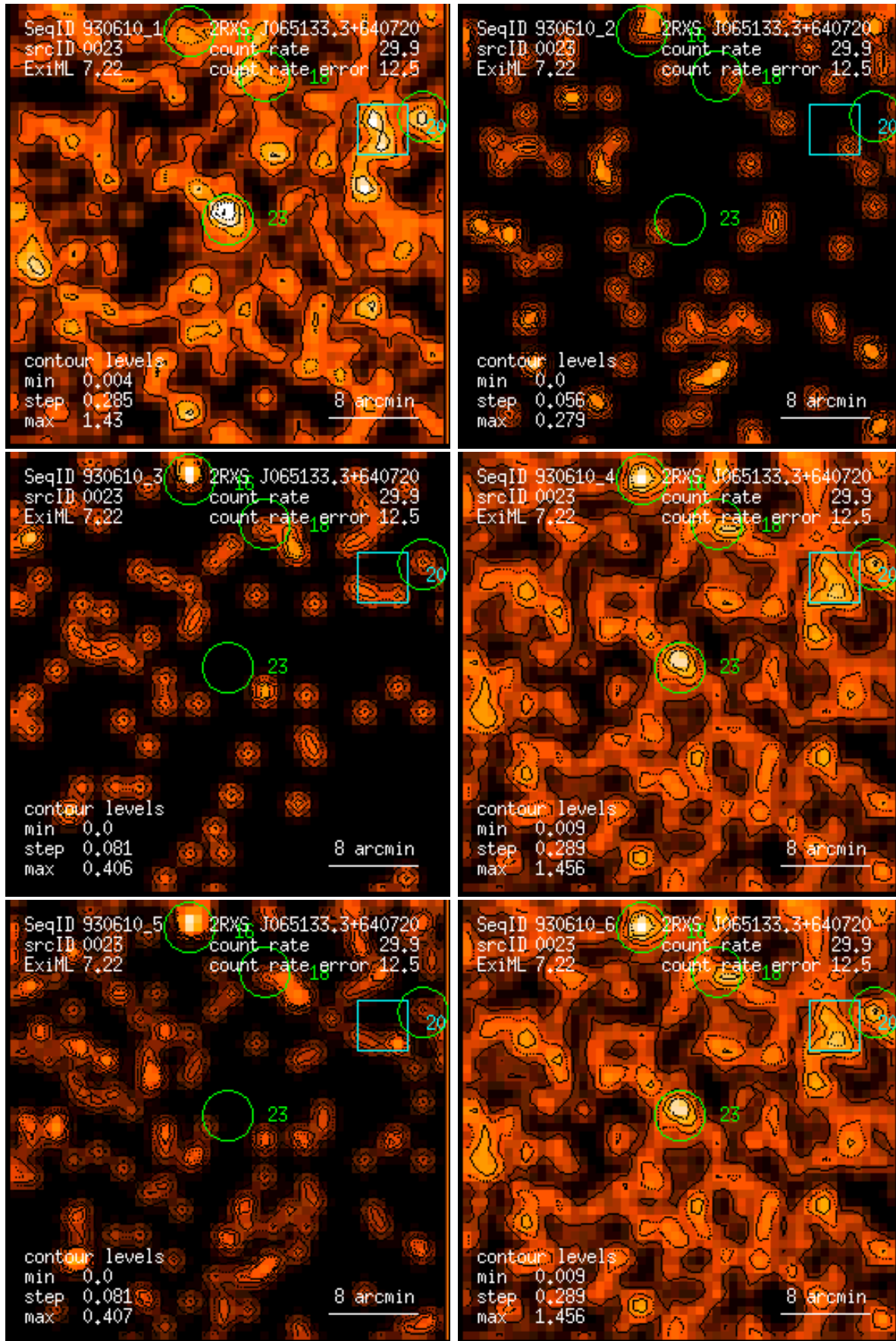
Figure 23: RASS 930610: detection 0023: band rate images, Gaussian filter: (1) PSPC channels 11 – 41, (2) 52 – 90, (3) 91 – 201, (4) 11 – 235, (5) 52 – 201, (6) 11 – 201. Broad band rates in counts/ks. Band rate contour levels in counts/ks/arcmin 2 .
