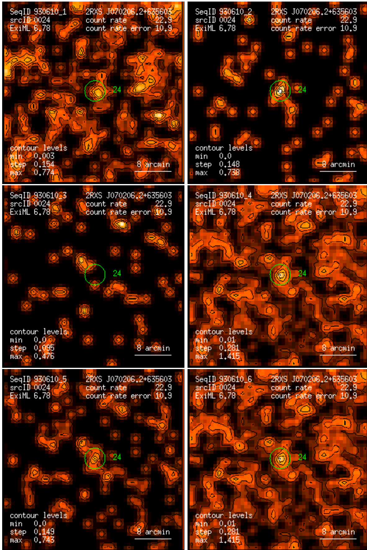
Figure 24: RASS 930610: detection 0024: band rate images, Gaussian filter: (1) PSPC channels 11 – 41, (2) 52 – 90, (3) 91 – 201, (4) 11 – 235, (5) 52 – 201, (6) 11 – 201. Broad band rates in counts/ks. Band rate contour levels in counts/ks/arcmin 2 .
