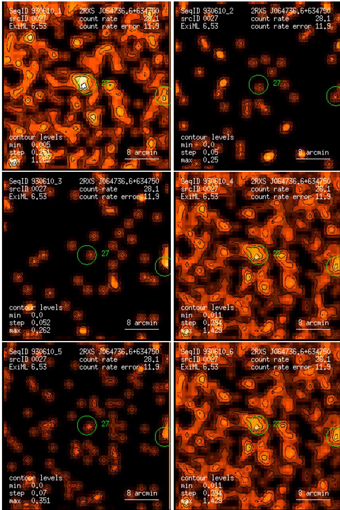
Figure 27: RASS 930610: detection 0027: band rate images, Gaussian filter: (1) PSPC channels 11 – 41, (2) 52 – 90, (3) 91 – 201, (4) 11 – 235, (5) 52 – 201, (6) 11 – 201. Broad band rates in counts/ks. Band rate contour levels in counts/ks/arcmin 2 .
