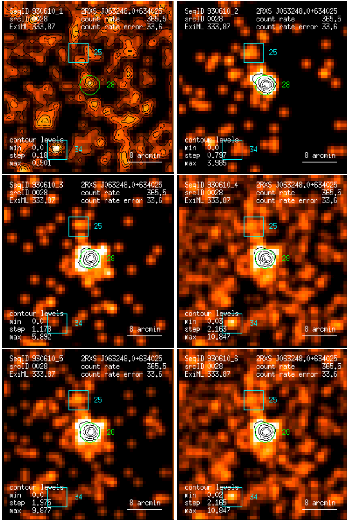
Figure 28: RASS 930610: detection 0028: band rate images, Gaussian filter: (1) PSPC channels 11 – 41, (2) 52 – 90, (3) 91 – 201, (4) 11 – 235, (5) 52 – 201, (6) 11 – 201. Broad band rates in counts/ks. Band rate contour levels in counts/ks/arcmin 2 .
