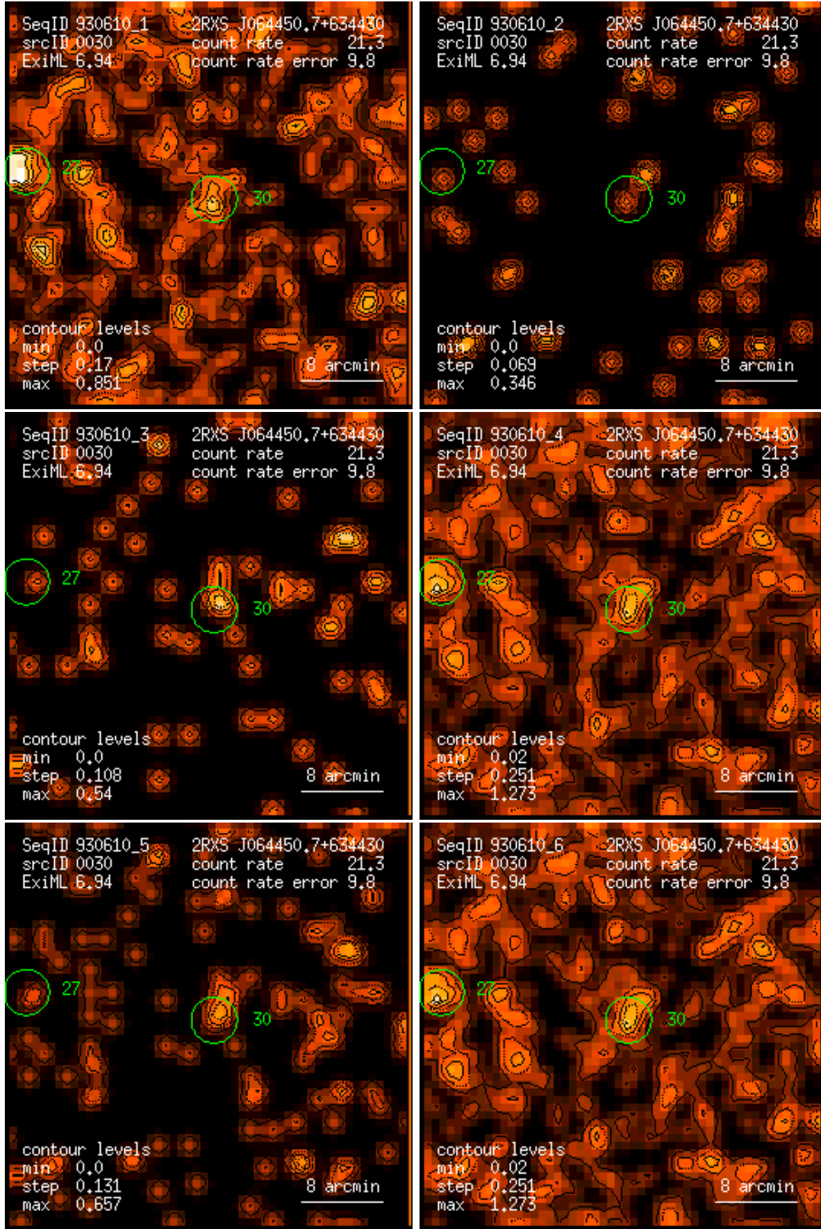
Figure 30: RASS 930610: detection 0030: band rate images, Gaussian filter: (1) PSPC channels 11 – 41, (2) 52 – 90, (3) 91 – 201, (4) 11 – 235, (5) 52 – 201, (6) 11 – 201. Broad band rates in counts/ks. Band rate contour levels in counts/ks/arcmin 2 .
