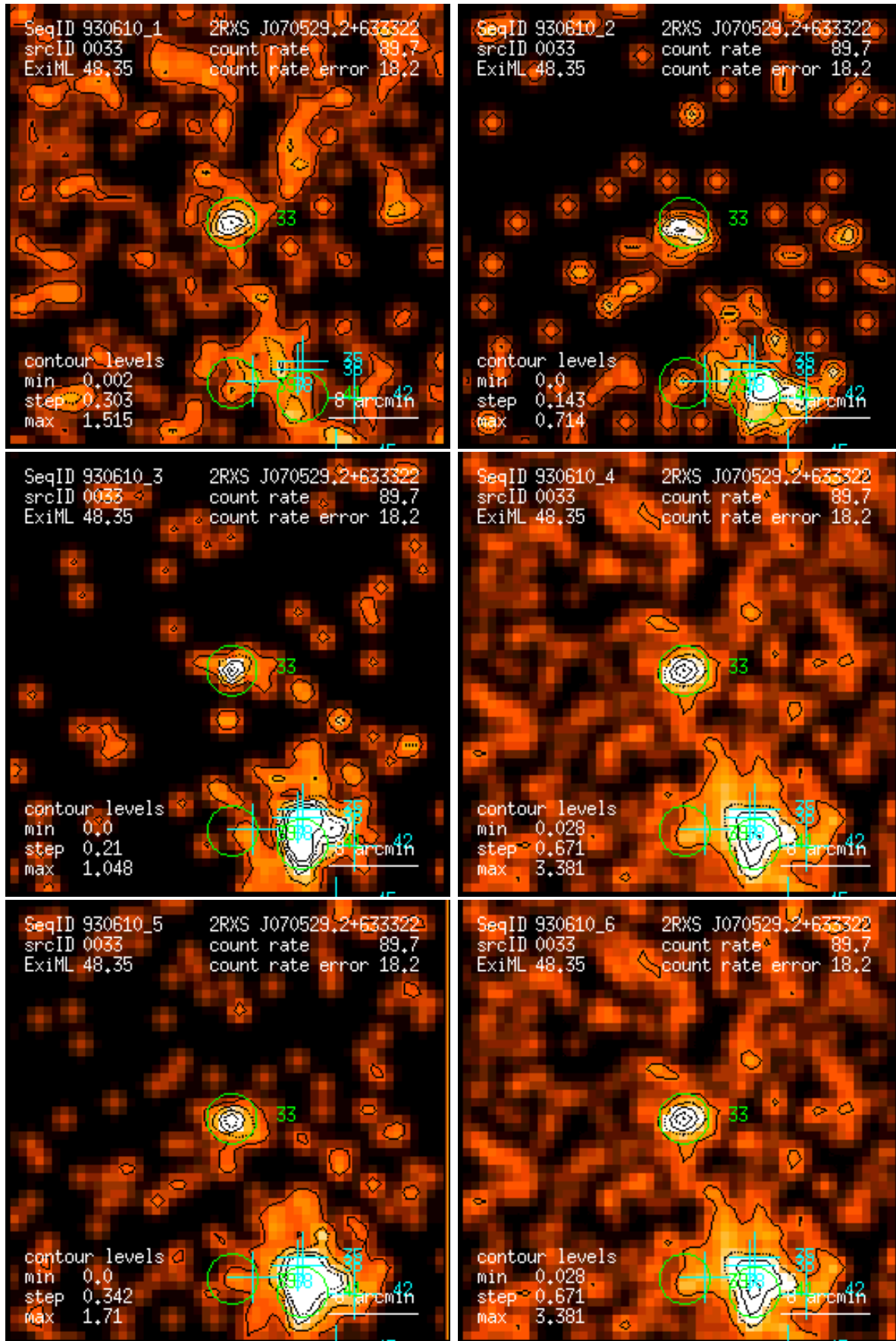
Figure 33: RASS 930610: detection 0033: band rate images, Gaussian filter: (1) PSPC channels 11 – 41, (2) 52 – 90, (3) 91 – 201, (4) 11 – 235, (5) 52 – 201, (6) 11 – 201. Broad band rates in counts/ks. Band rate contour levels in counts/ks/arcmin 2 .
