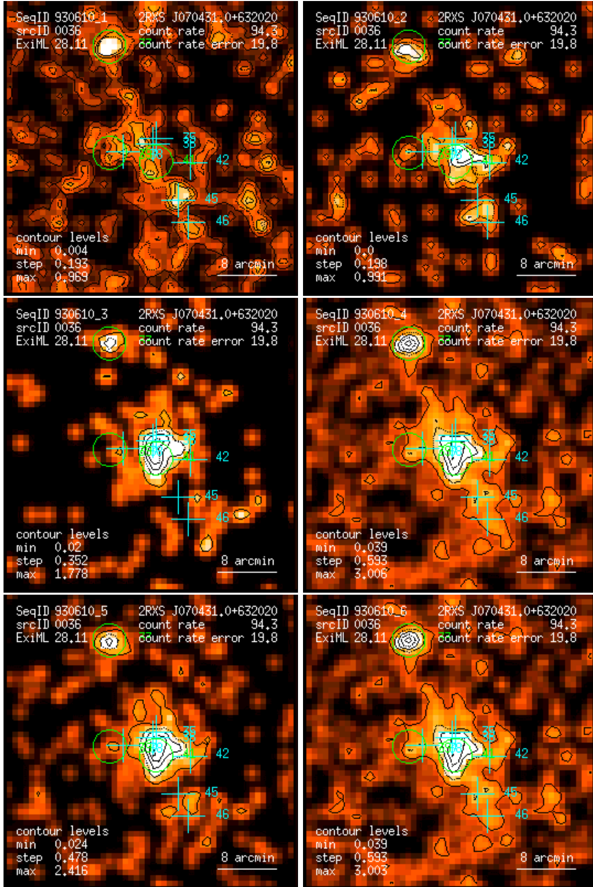
Figure 36: RASS 930610: detection 0036: band rate images, Gaussian filter: (1) PSPC channels 11 – 41, (2) 52 – 90, (3) 91 – 201, (4) 11 – 235, (5) 52 – 201, (6) 11 – 201. Broad band rates in counts/ks. Band rate contour levels in counts/ks/arcmin 2 .
